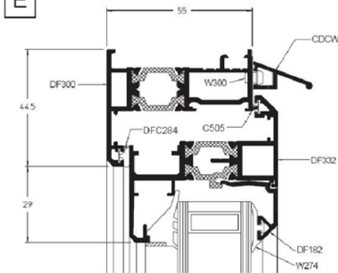
E Head / Vent
