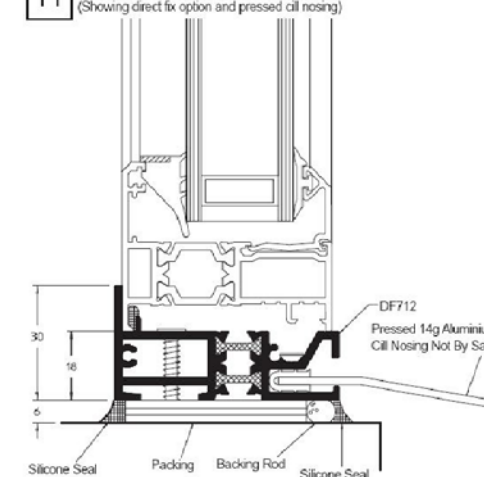
H Subcill / Fixed Light (Showing direct fix option and pressed cill nosing)
