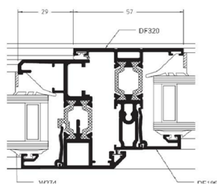
B Mullion / Vent
