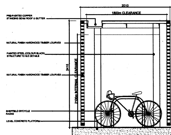
2 PROPOSED CYCLE STORE SECTION 1:50
