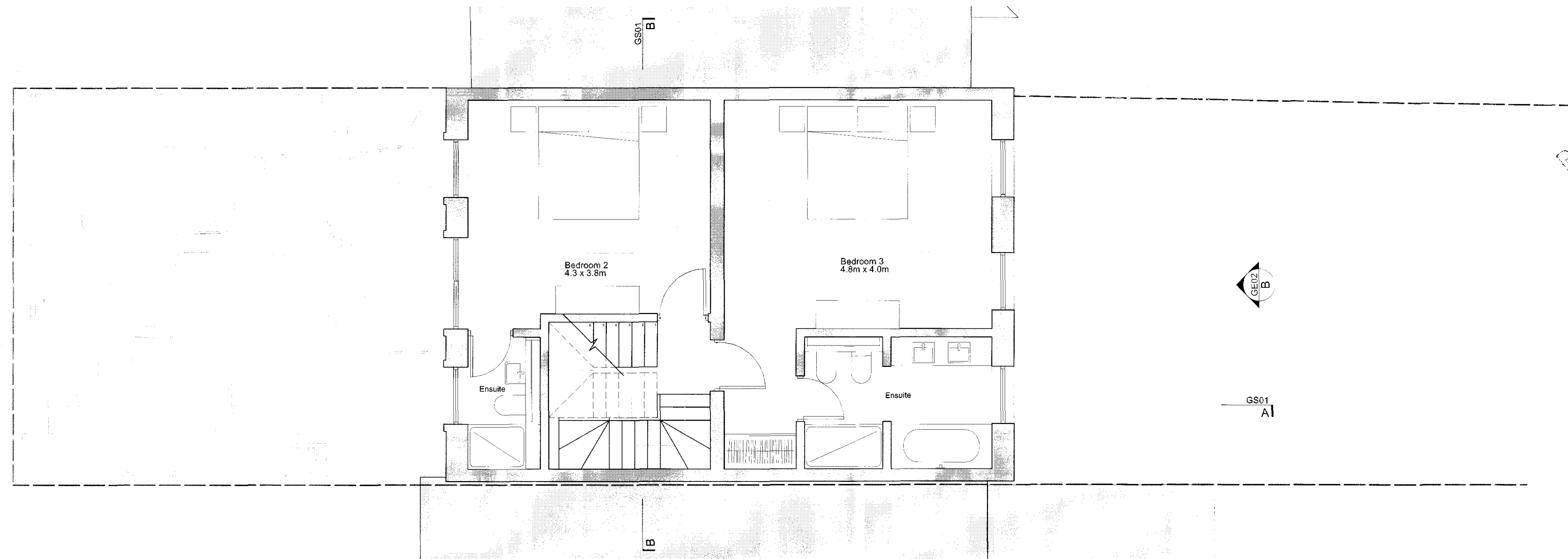
B Proposed First Floor 1:100 @ A3
