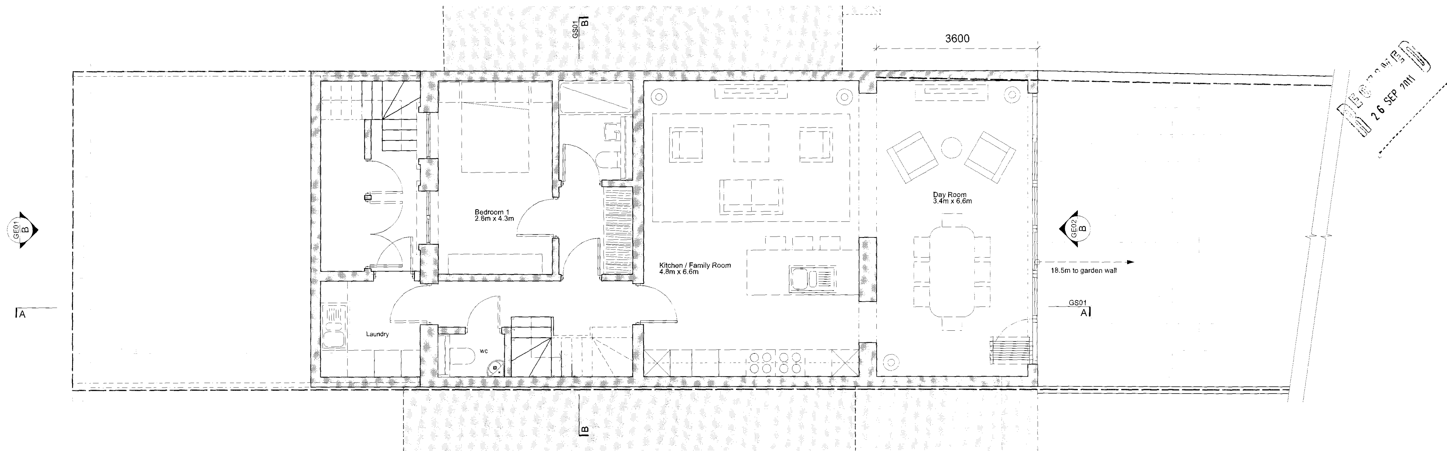
B Proposed Lower Ground 1:100 @ A3
