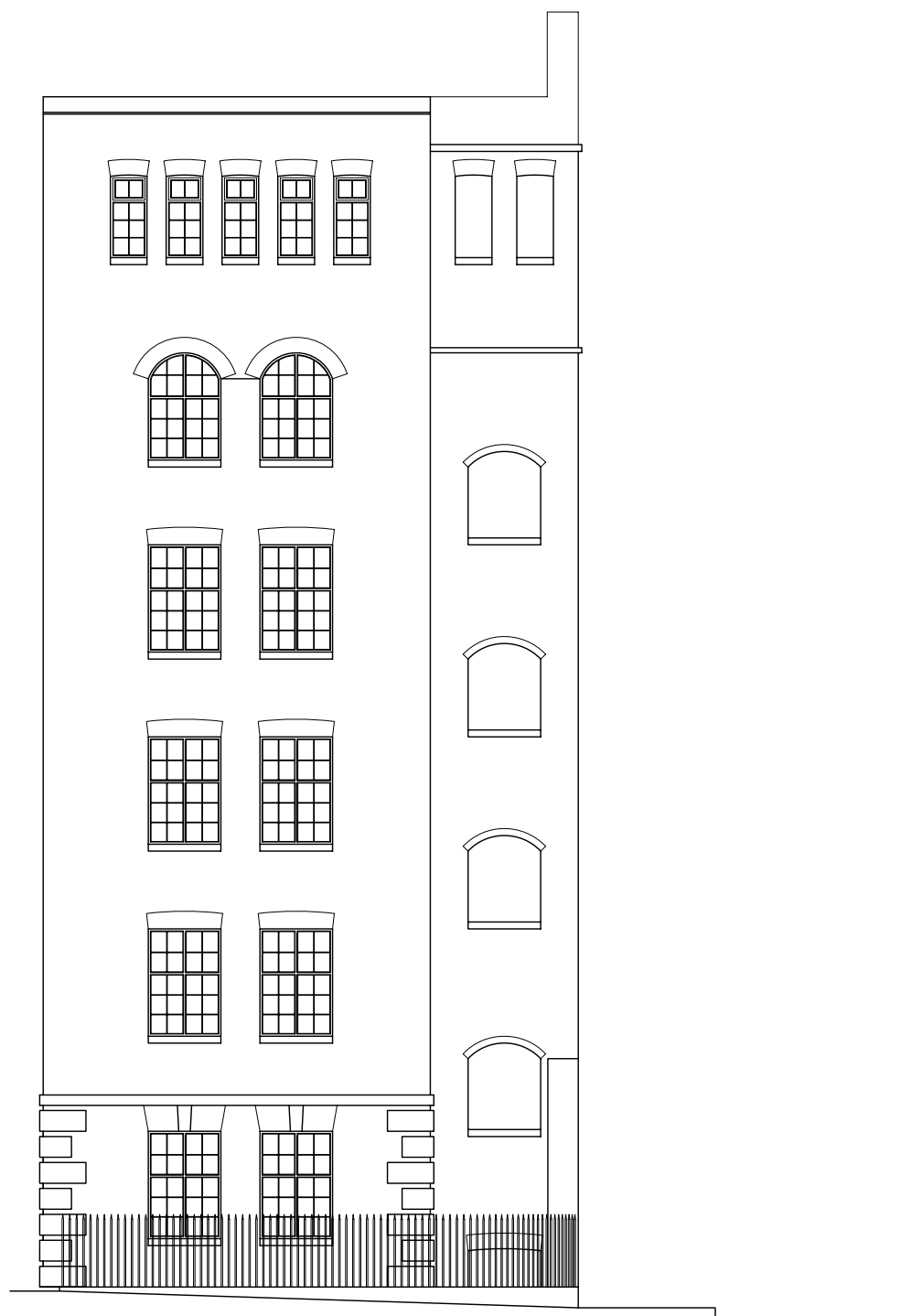
EXISTING SOUTH EAST ELEVATION
