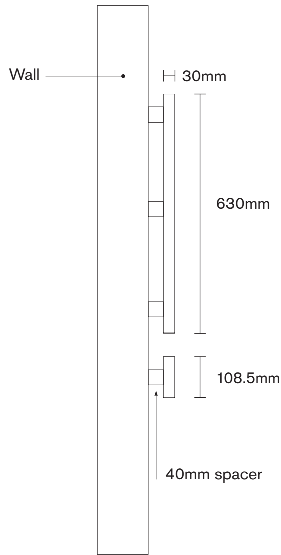
Side elevation
