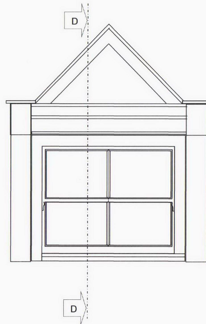
FRONT ELEVATION SHOWING PROPOSED OUTER BOX SASH WINDOWS
