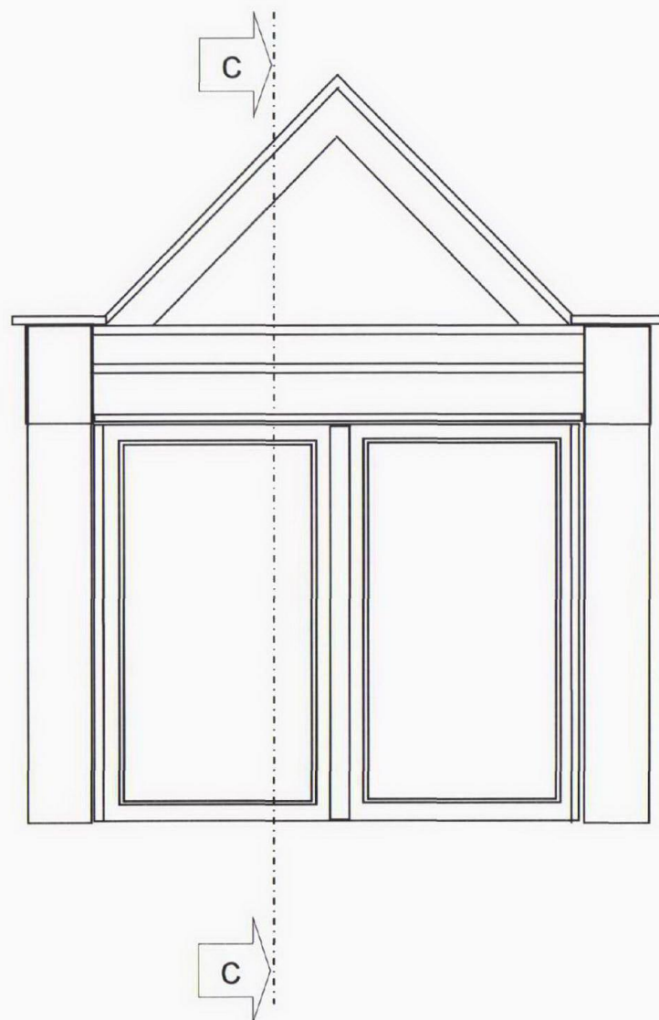
FRONT ELEVATION SHOWING EXISTING OUTER TIMBER CASEMENT WINDOWS
