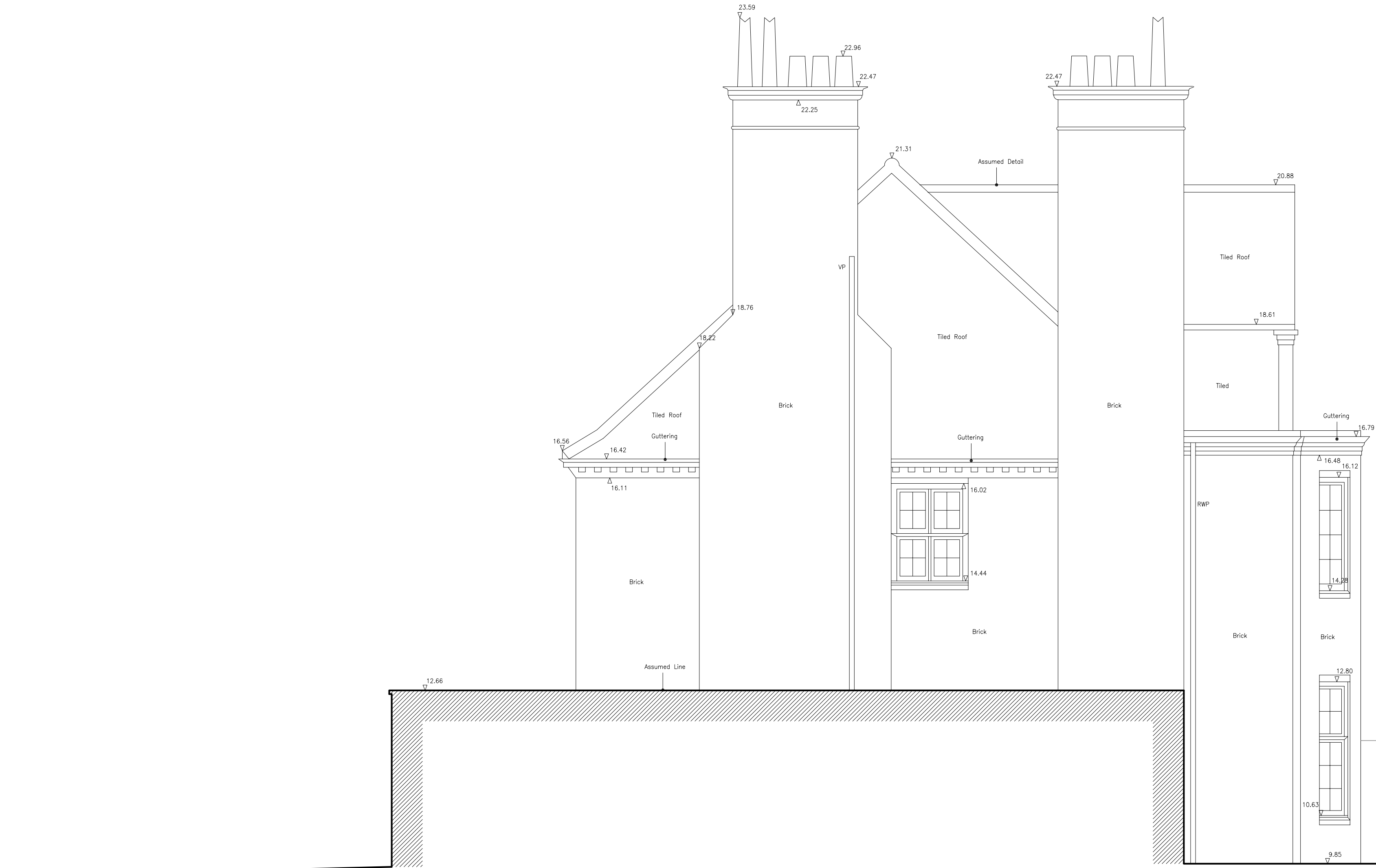
SIDE ELEVATION (WEST)
