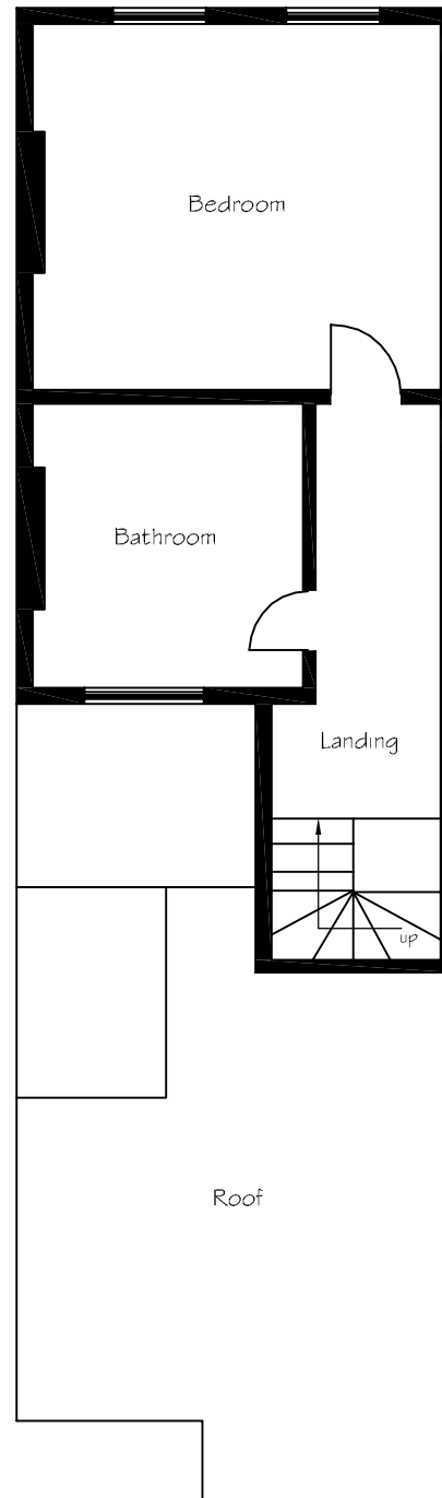
First Floor
