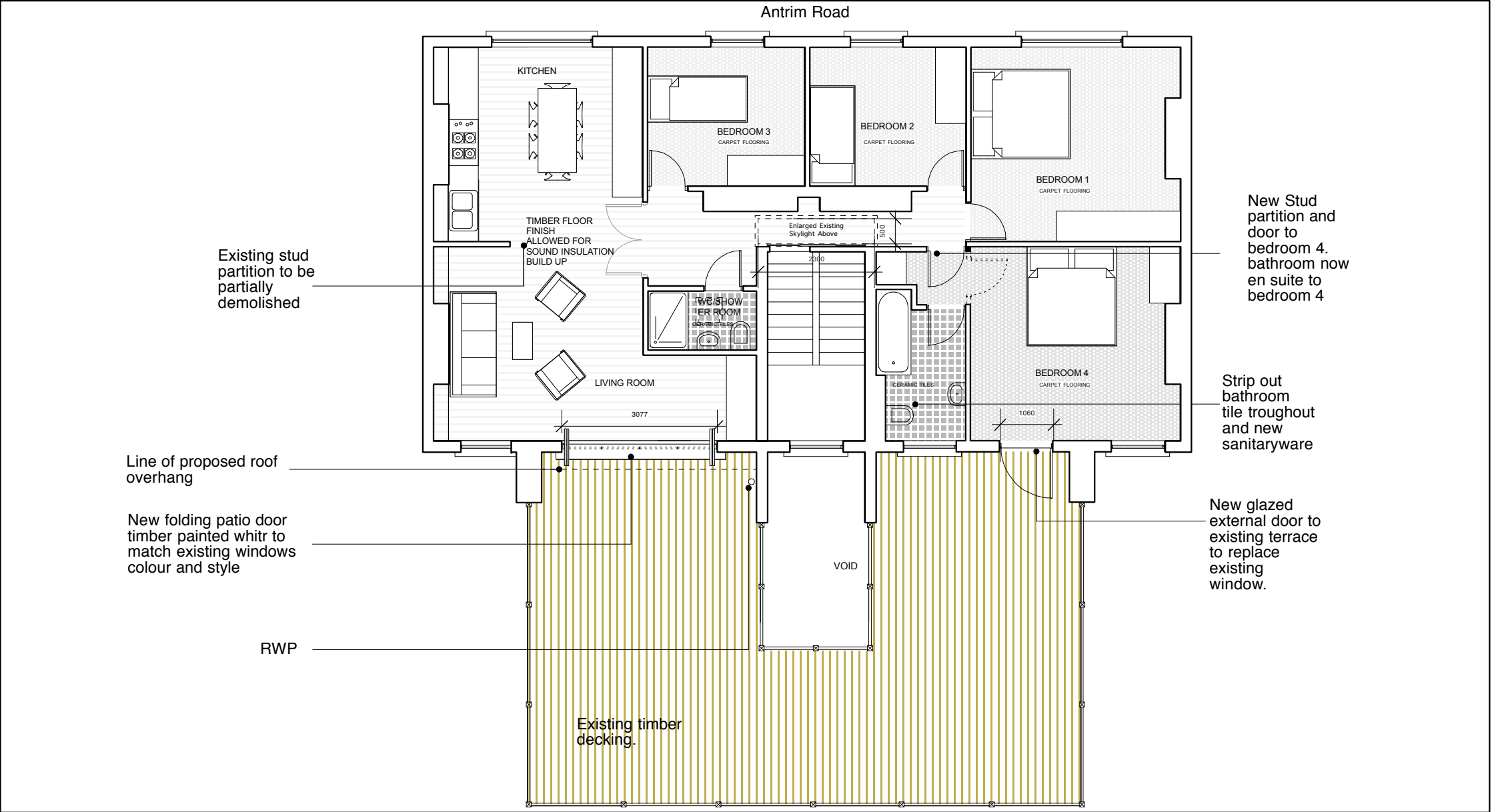
PROPOSED FLOOR PLAN SCALE 1:100 @ A3
