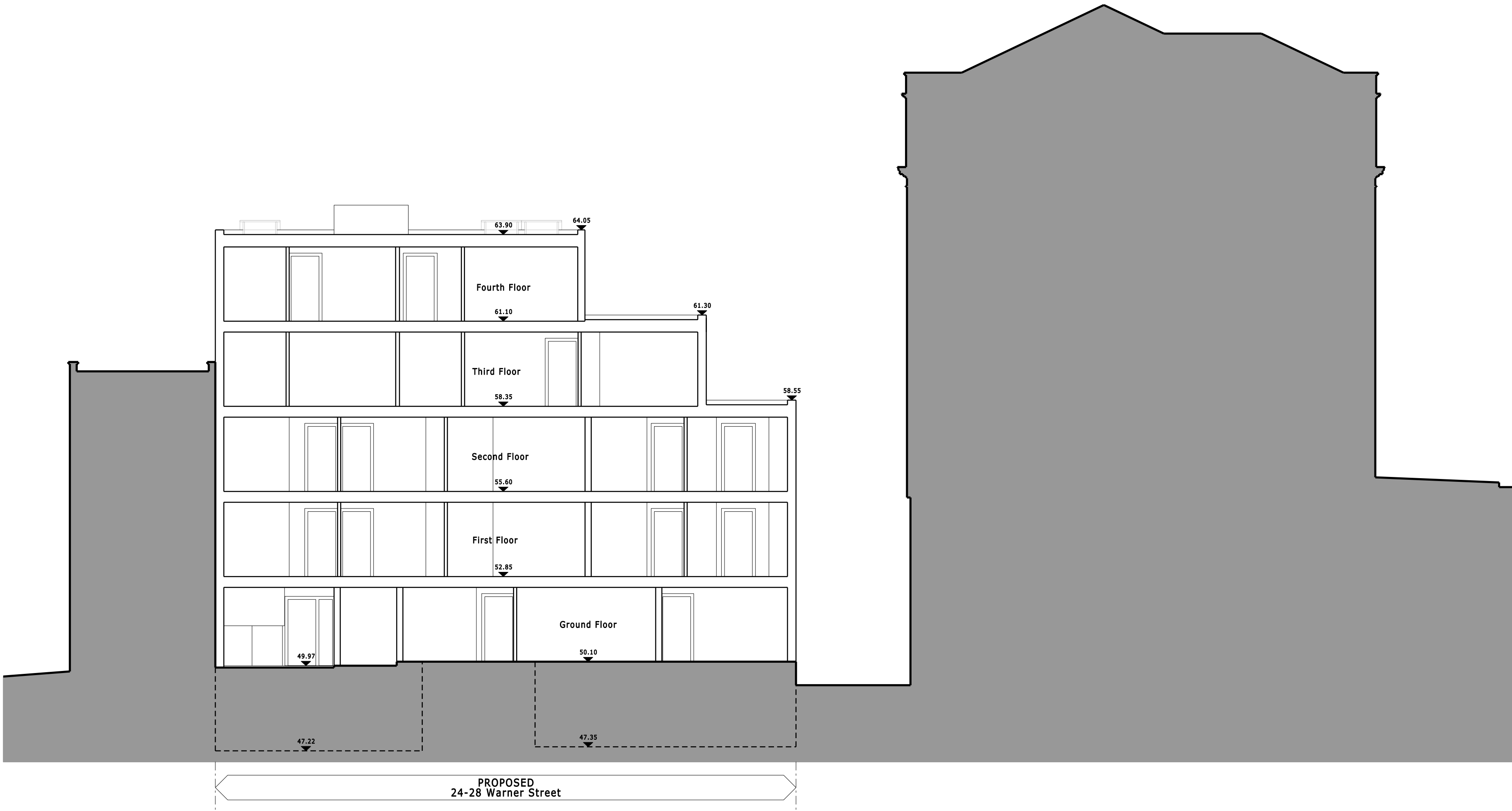
SECTION E-E
