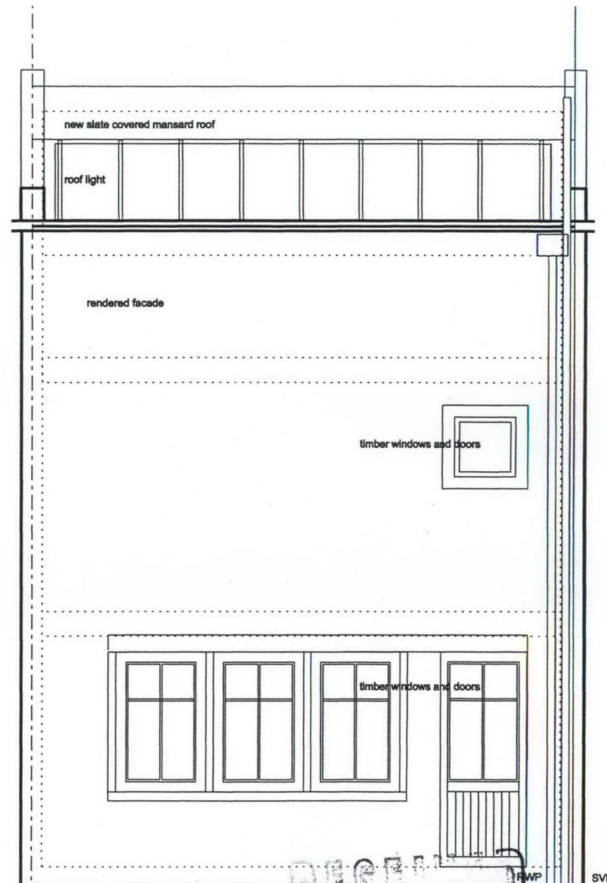
REAR ELEVATION
