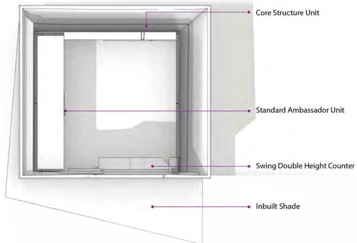
Plan View Roof of Core Structure Removed
