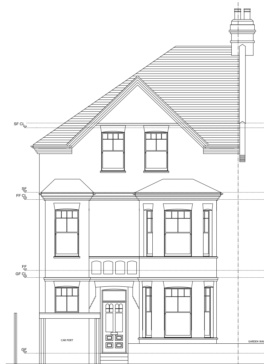
STREET ELEVATION
