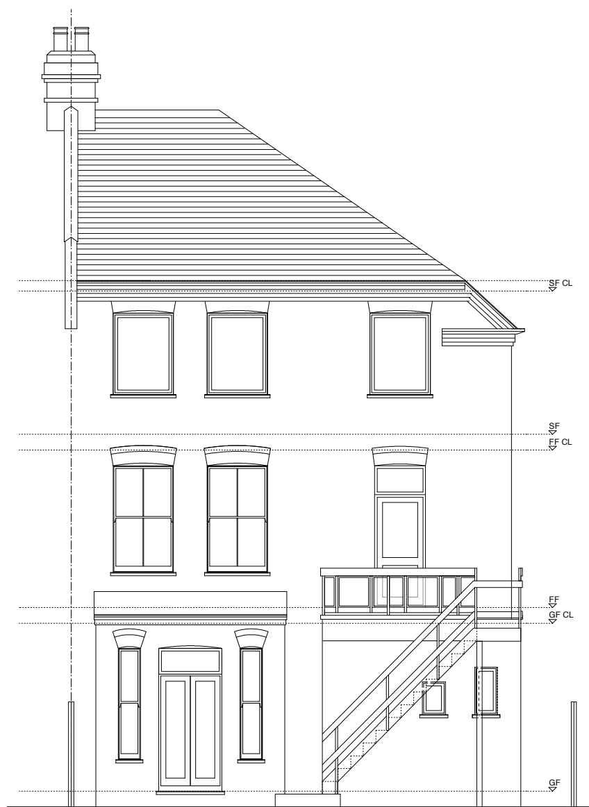
REAR ELEVATION
