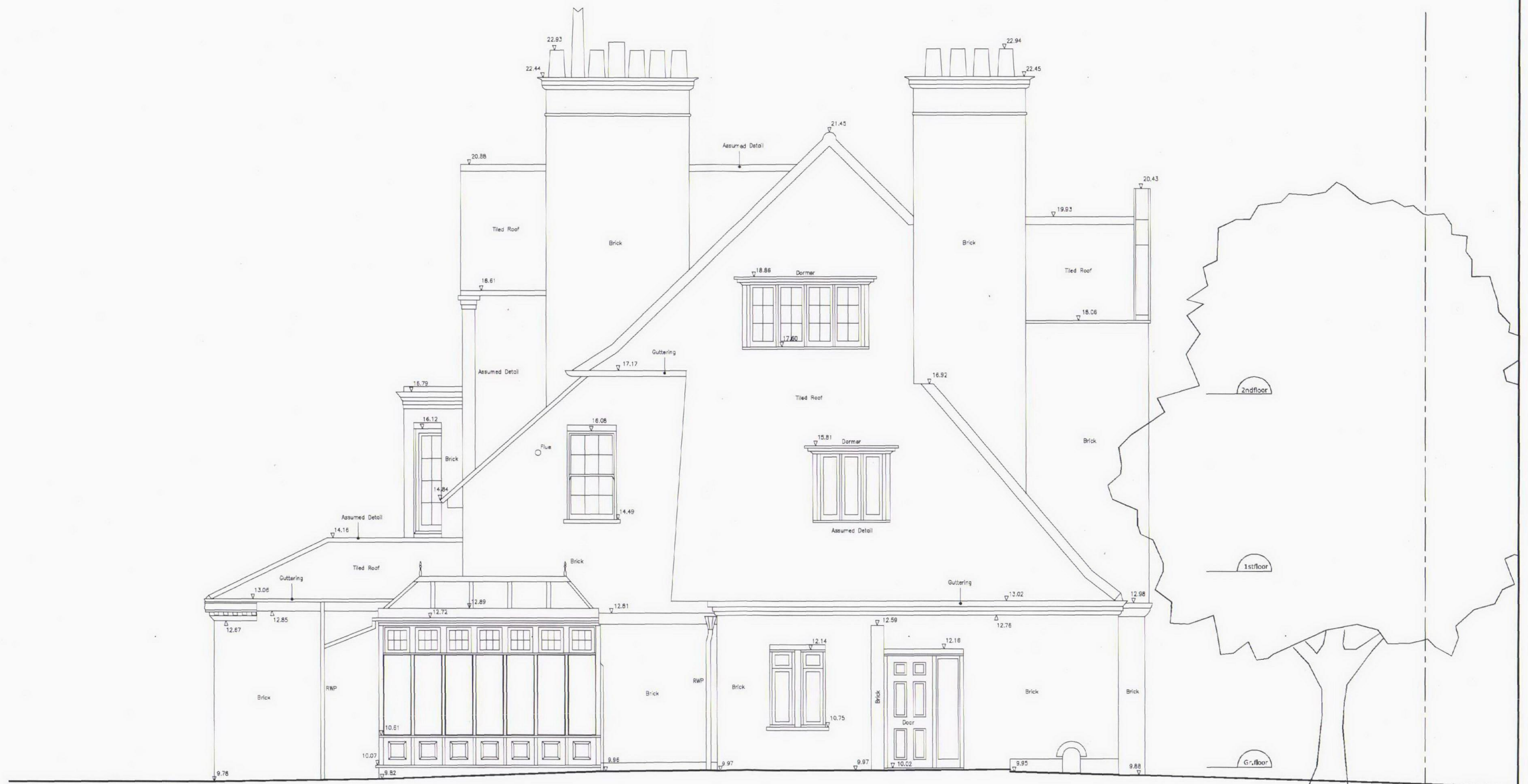
SIDE ELEVATION (EAST)
