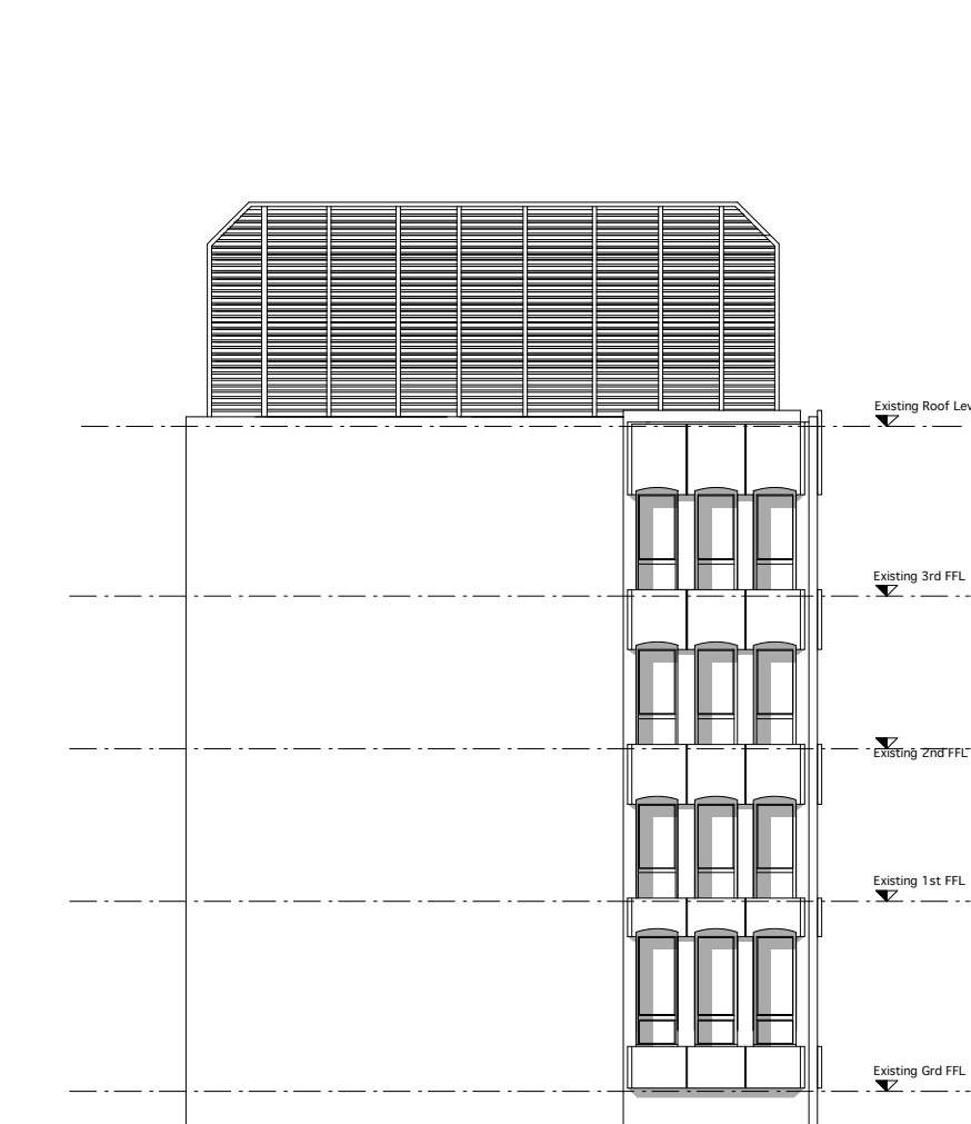
EXISTING SOUTH EAST ELEVATION A
