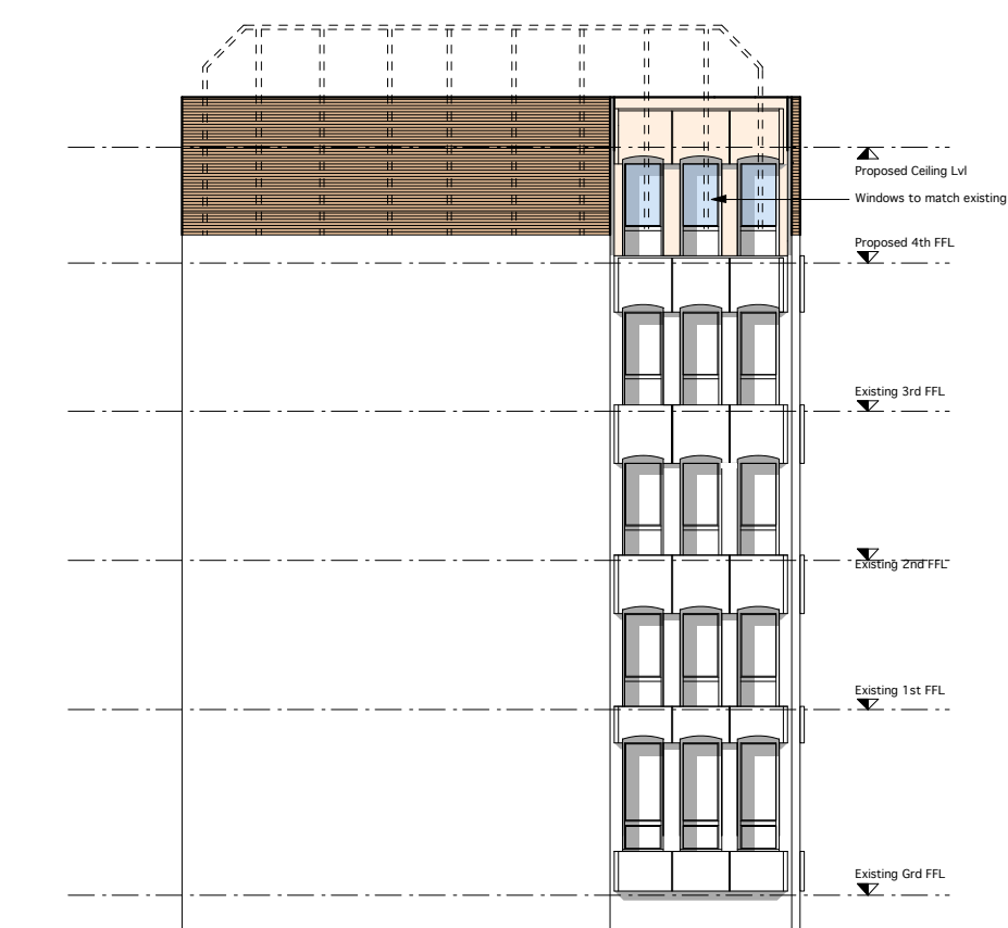
PROPOSED SOUTH EAST ELEVATION A
