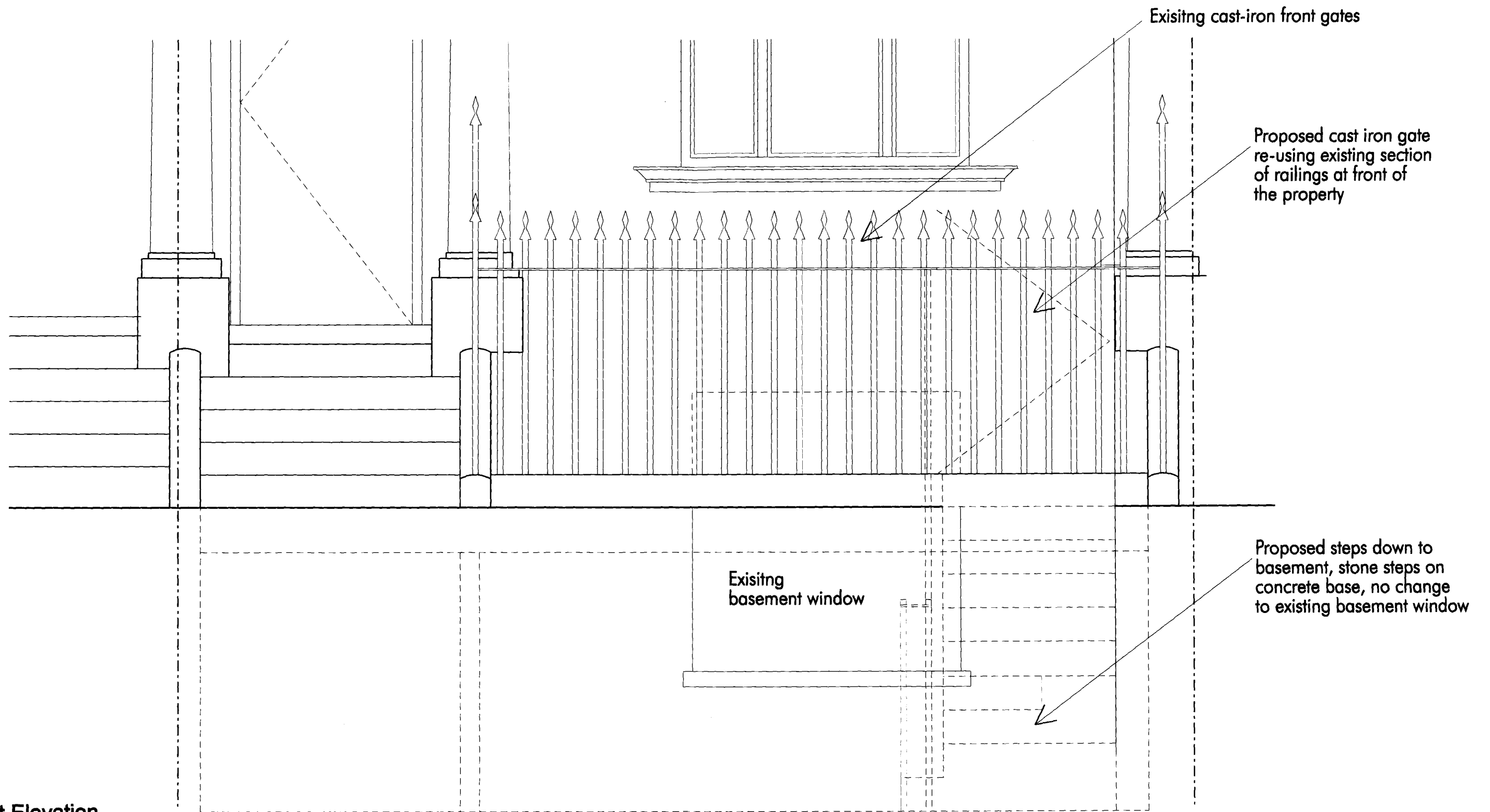
Front Elevation
