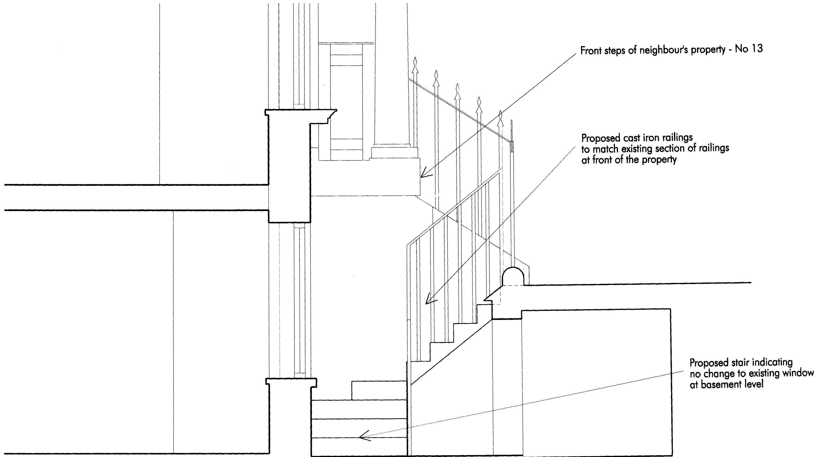
Section AA
