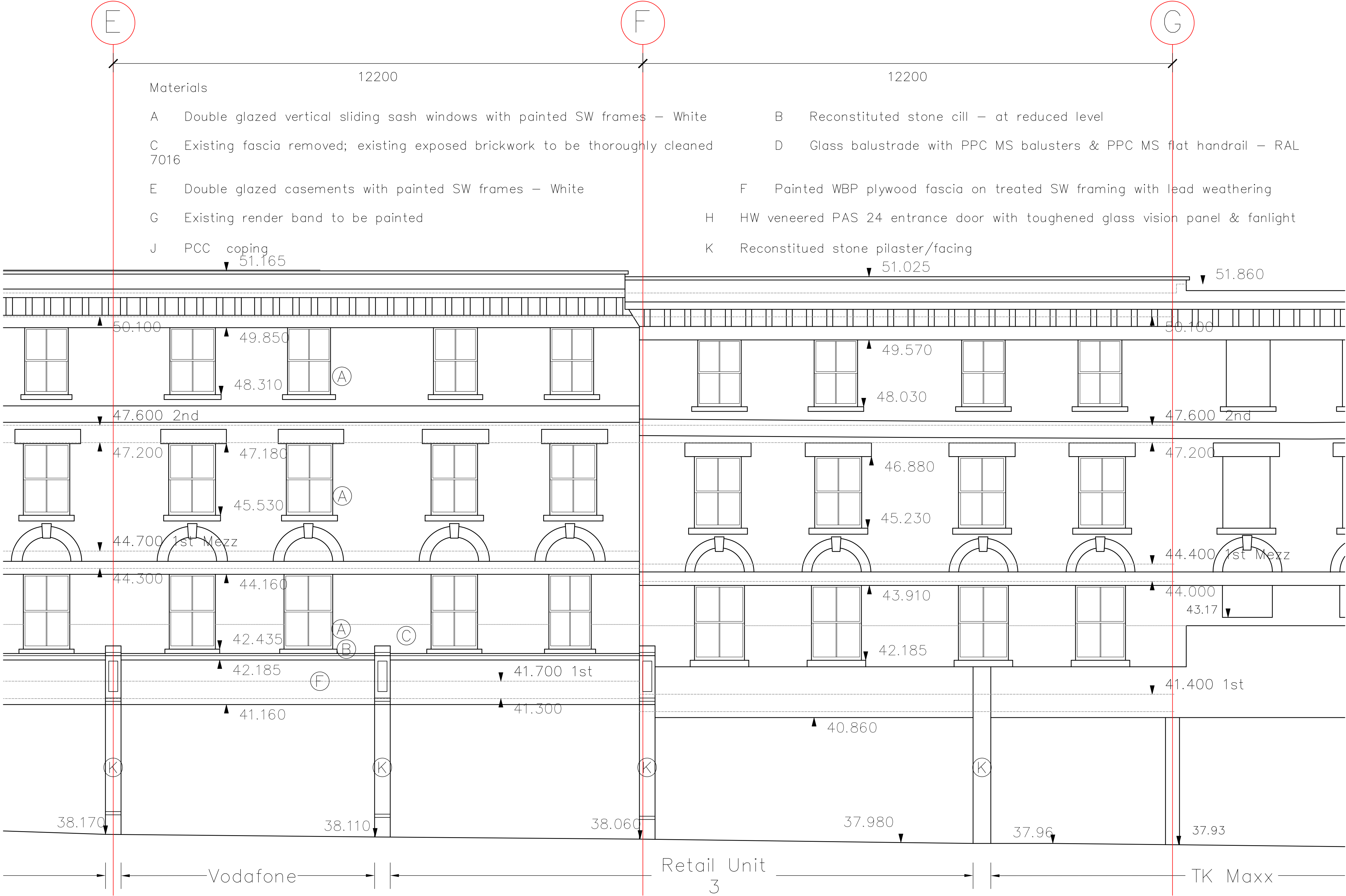
Kilburn High Road Elevation
