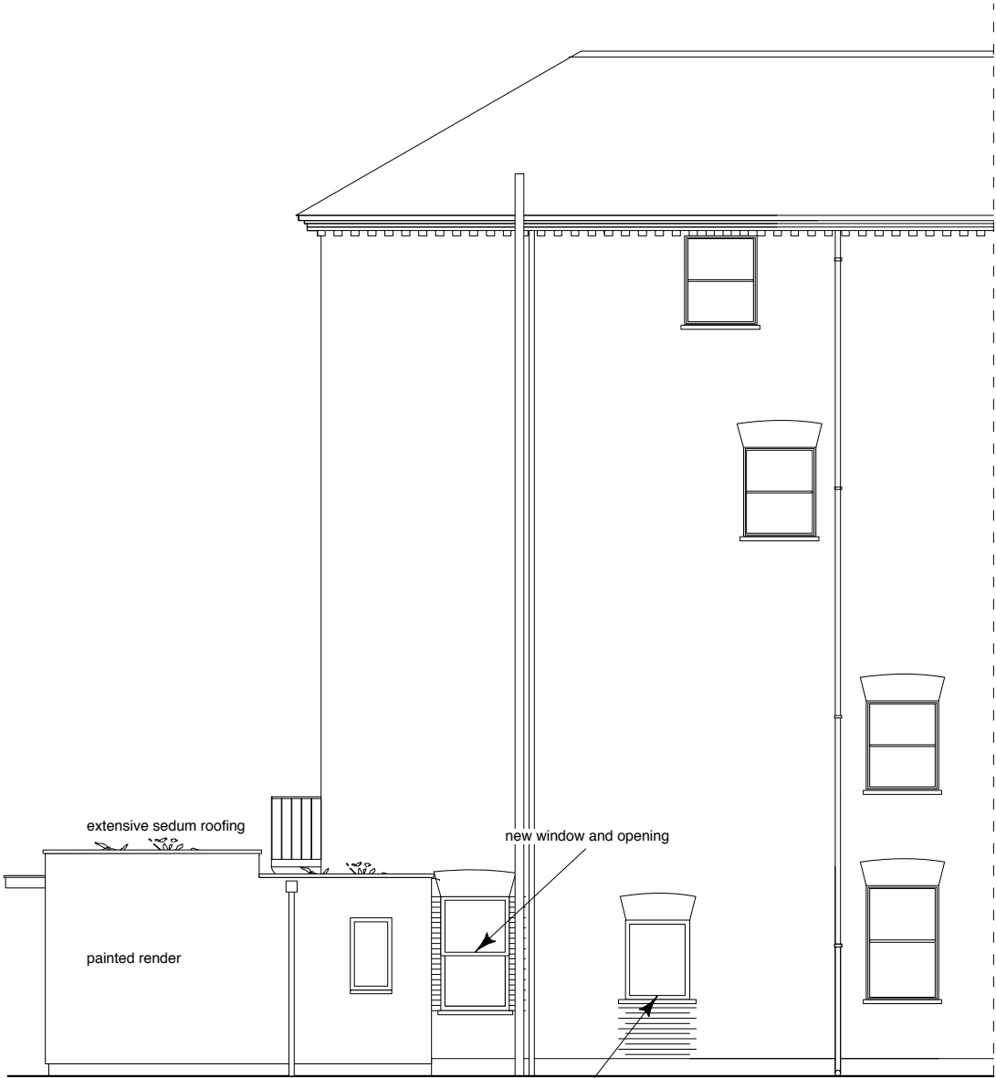
north elevation
