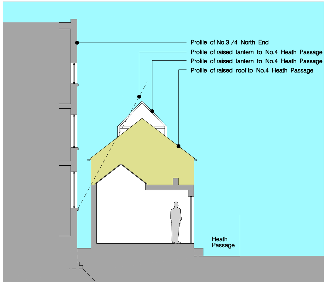
Section A–A: As proposed
