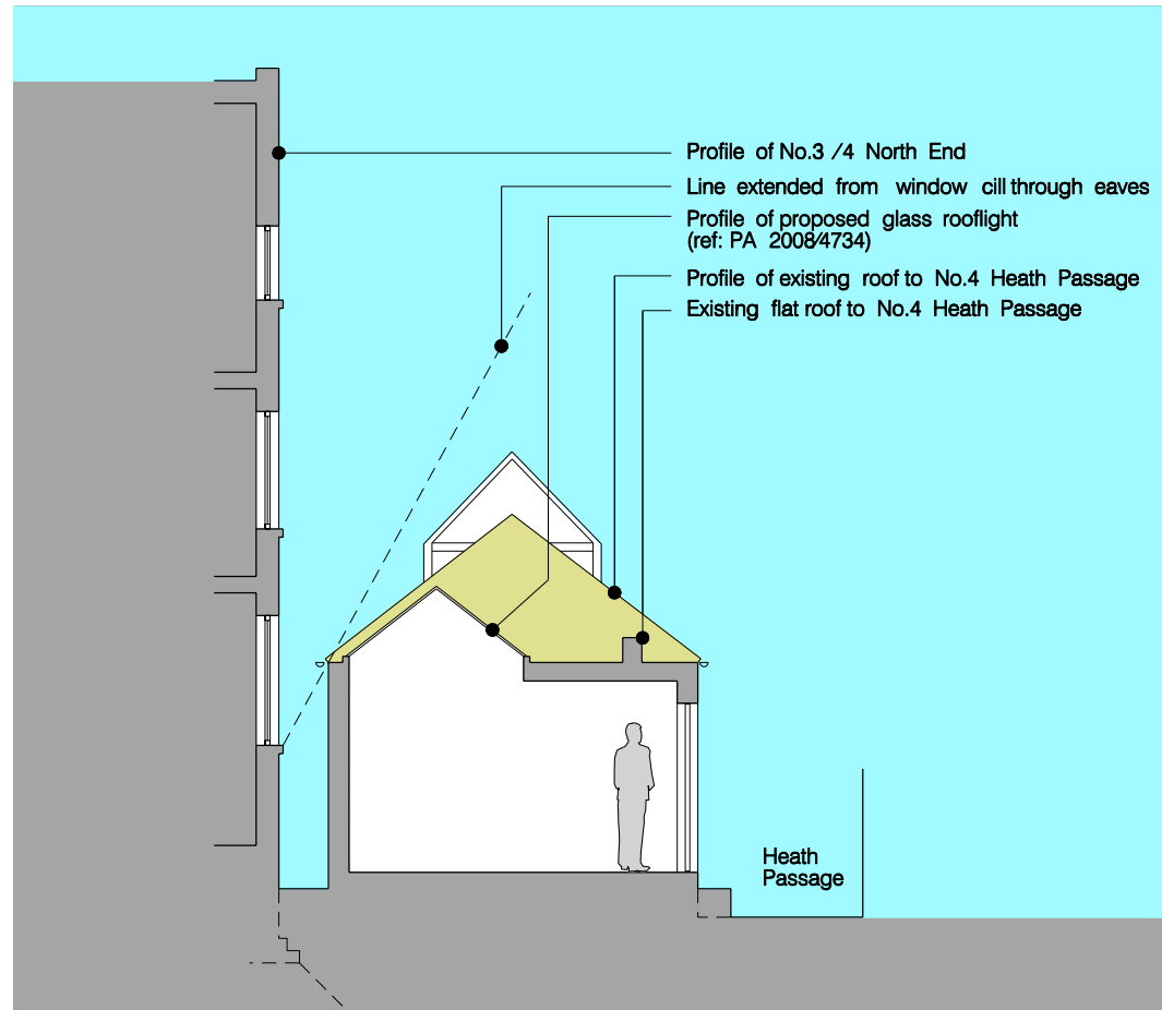
Section A–A: As existing
