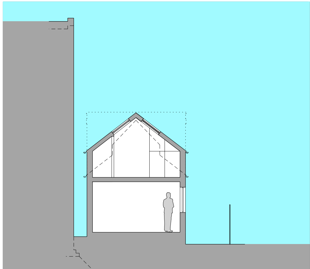
Section B–B: As proposed
