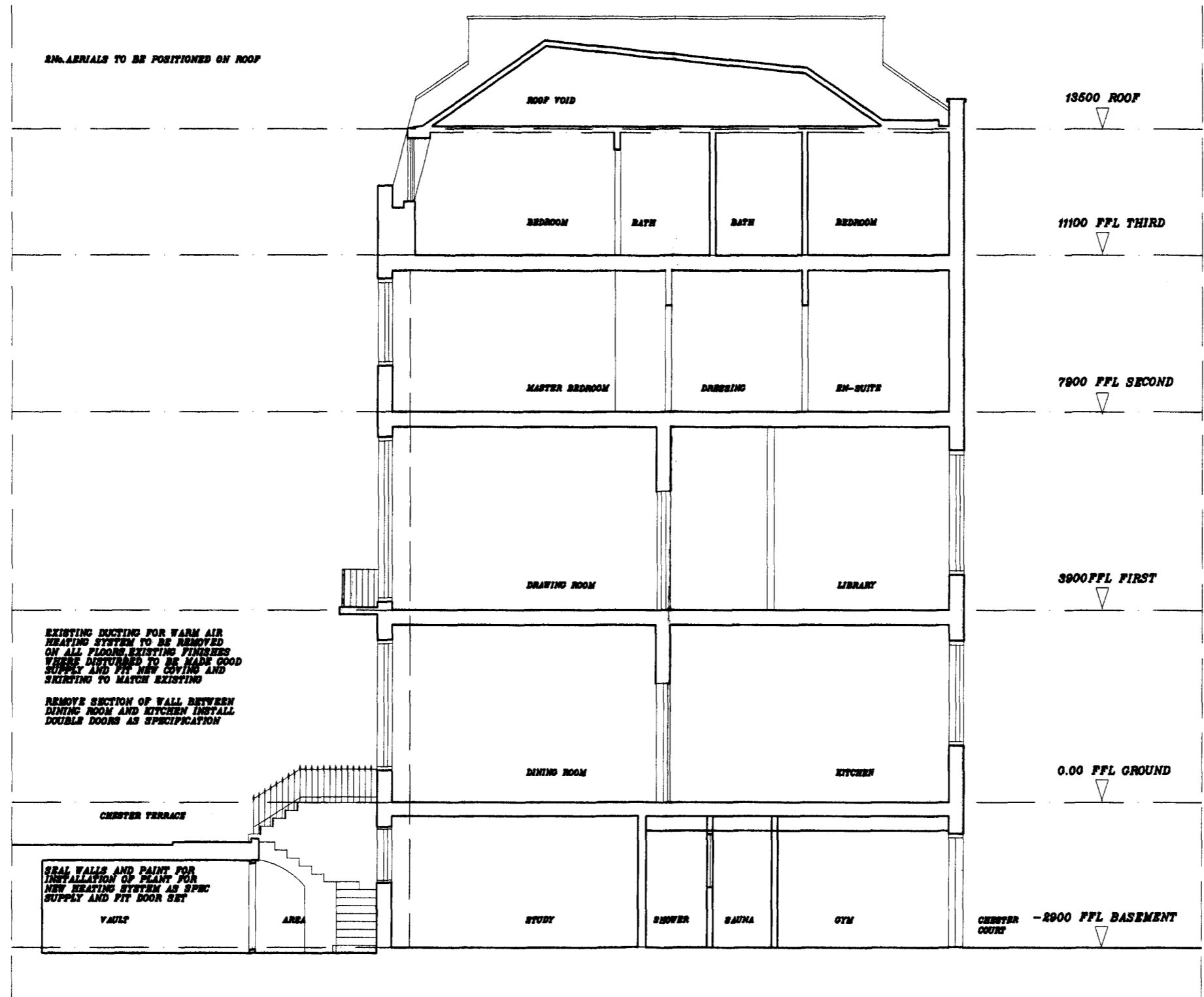
EXISTING SECTION
