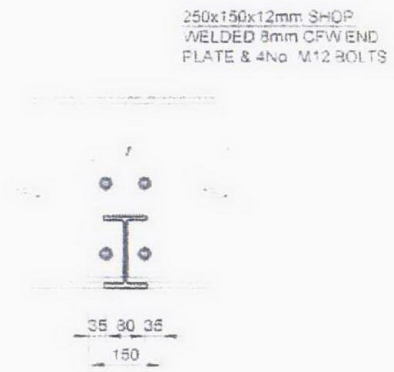
152 UB TO 406 UB WEB CONNECTION. SECTION THROUGH 152 UB 1 10 @ A1
