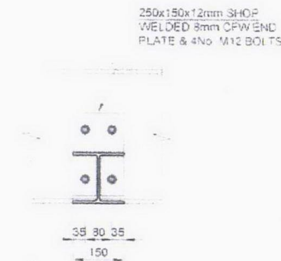
152 UC TO 406 UB WEB CONNECTION. SECTION THROUGH 152 UC 1 10 @ A1
