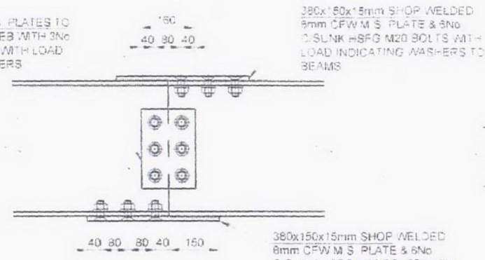
406x178 UB 60 SPLICE ELEVATION 1 10 @ A1
