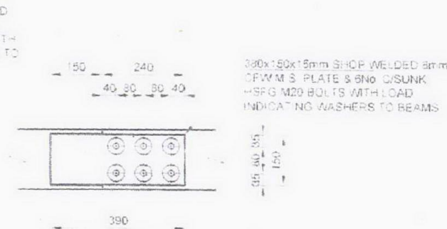
406x178 UB 60 PLAN SPLICE 1 10 @ A1
