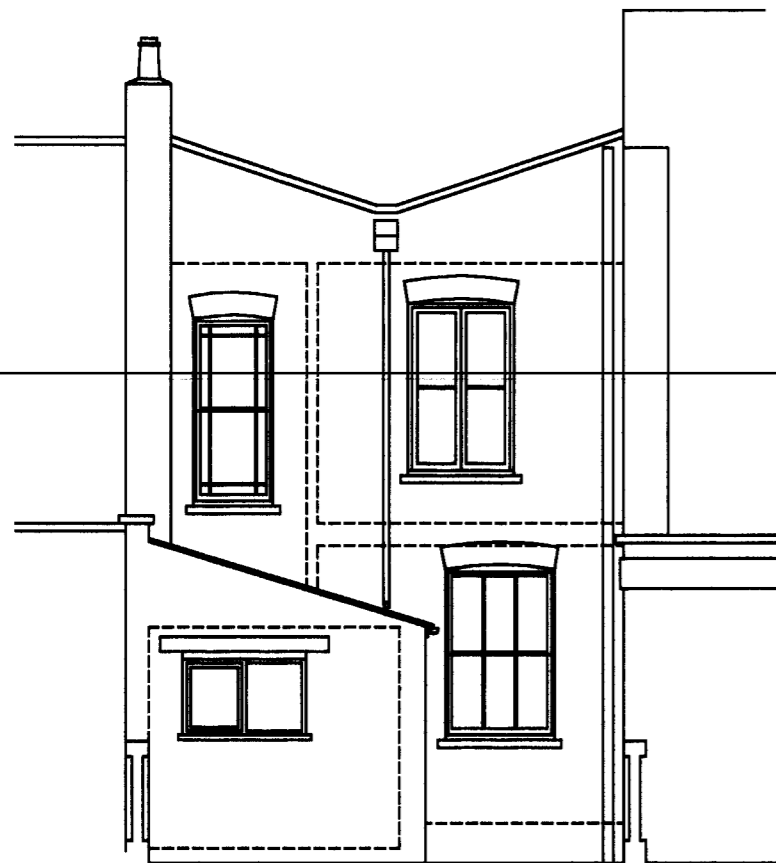
REAR ELEVATION
