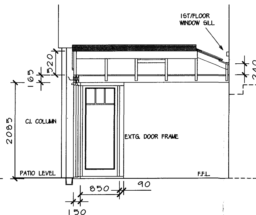
PROPOSED SECTION
