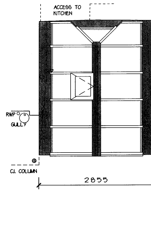
PROPOSED ROOF
