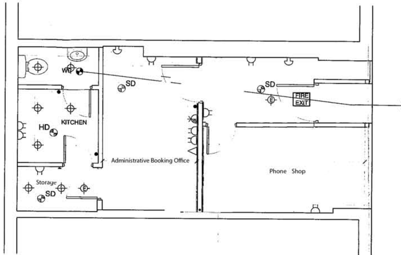
PROPOSED plan @ 1:50
