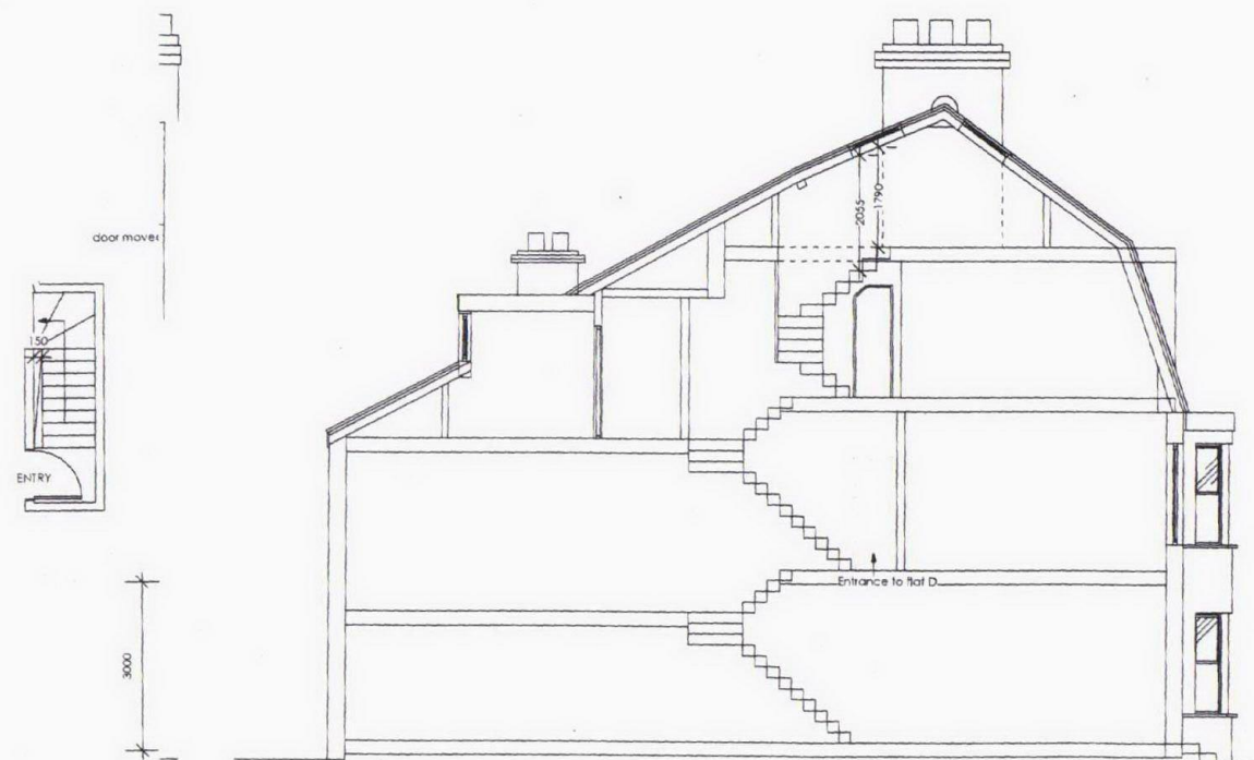
PROPOSED SECTION
