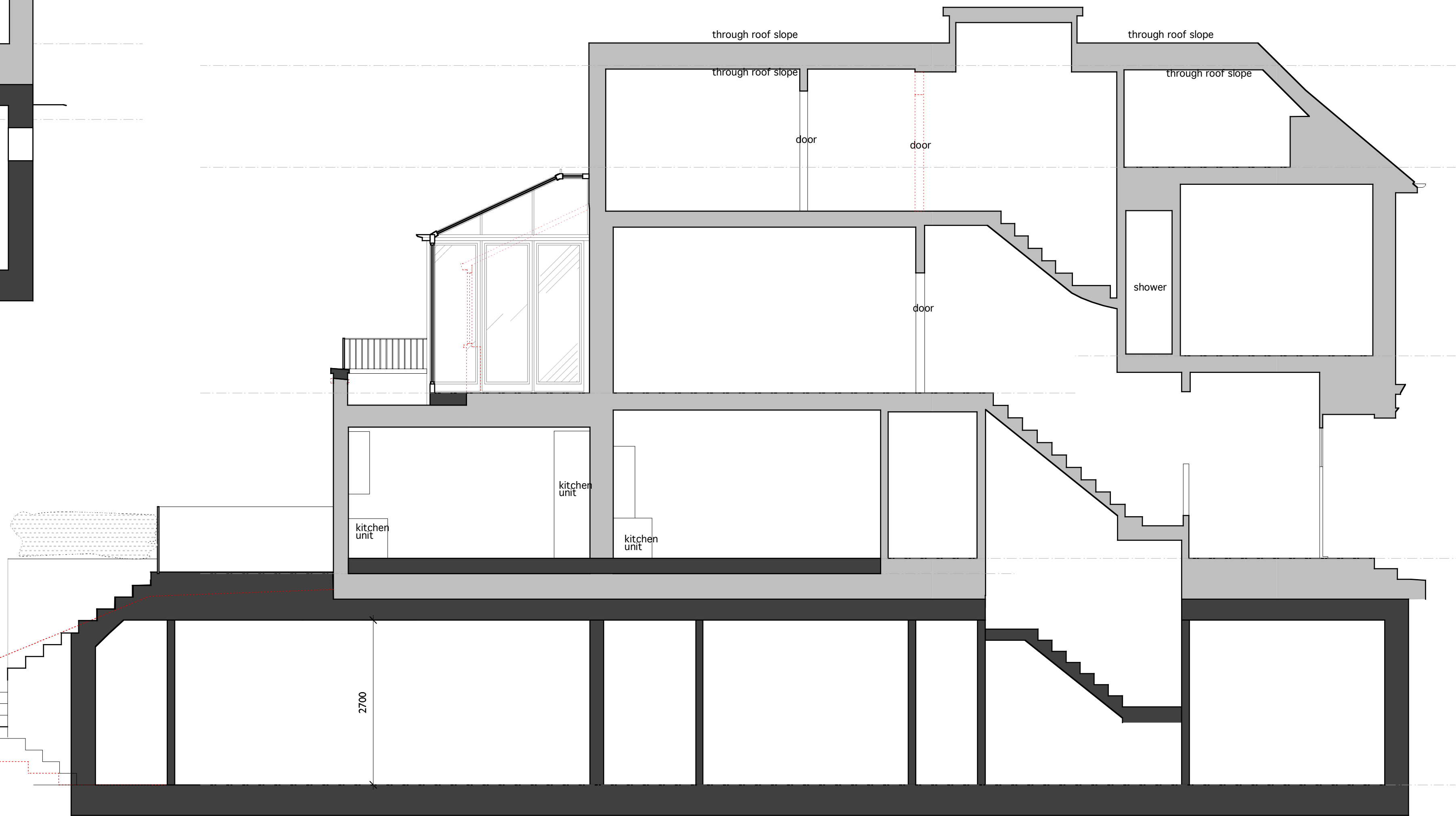
PROPOSED SECTION AA
