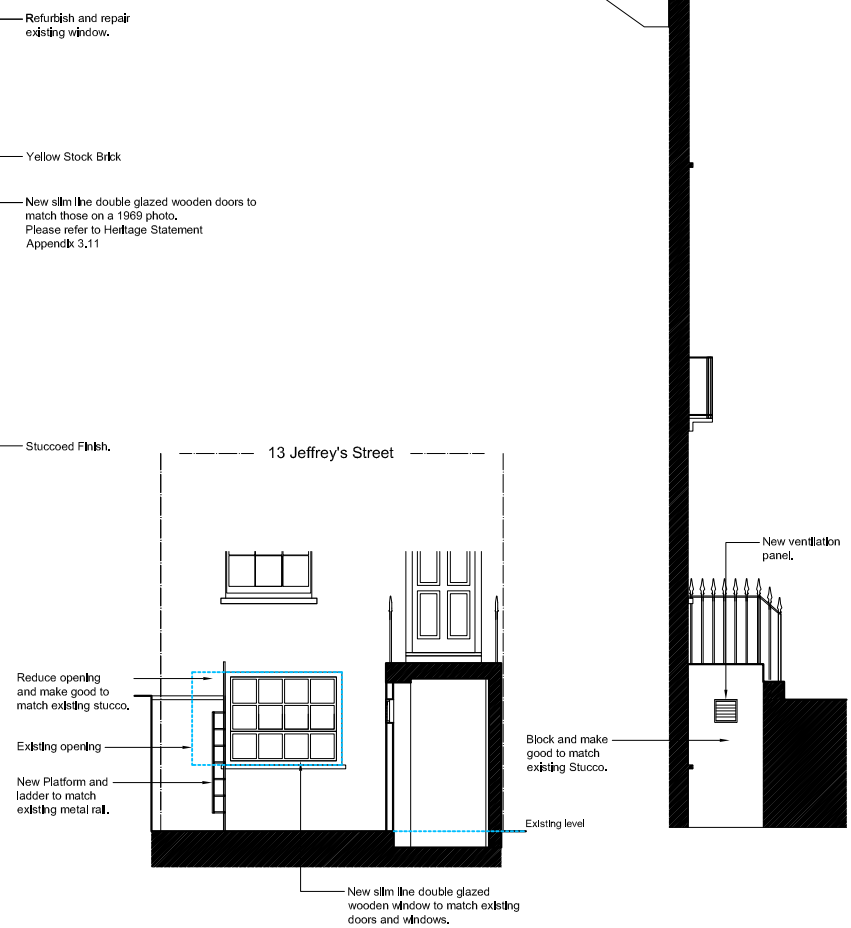
Front Elevation/ Section Basement Level
