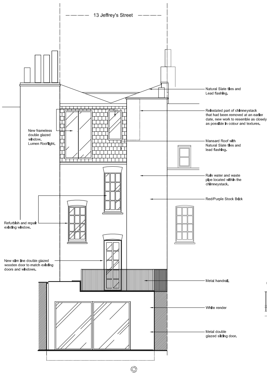
Back Elevation
