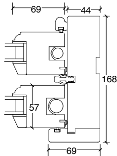
DETAIL SECTION C-C SCALE 1:5
