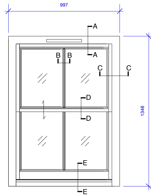
TYPE C (2 No.) Timber frame. 2 x 4mm glazing with 16mm cavity.
