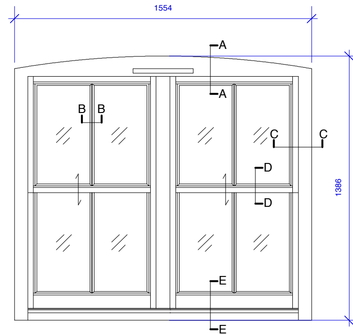
TYPE A (2 No.) Timber frame. 2 x 4mm glazing with 16mm cavity.
