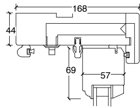
DETAIL SECTION A-A SCALE 1:5
