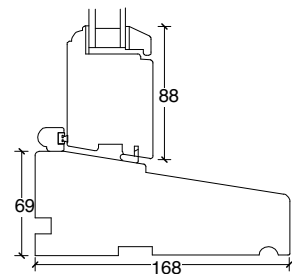
DETAIL SECTION E-E SCALE 1:5
