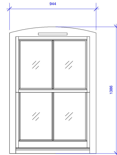
TYPE B (1 No.) Timber frame. Obscure double glazing. Non-opening.
