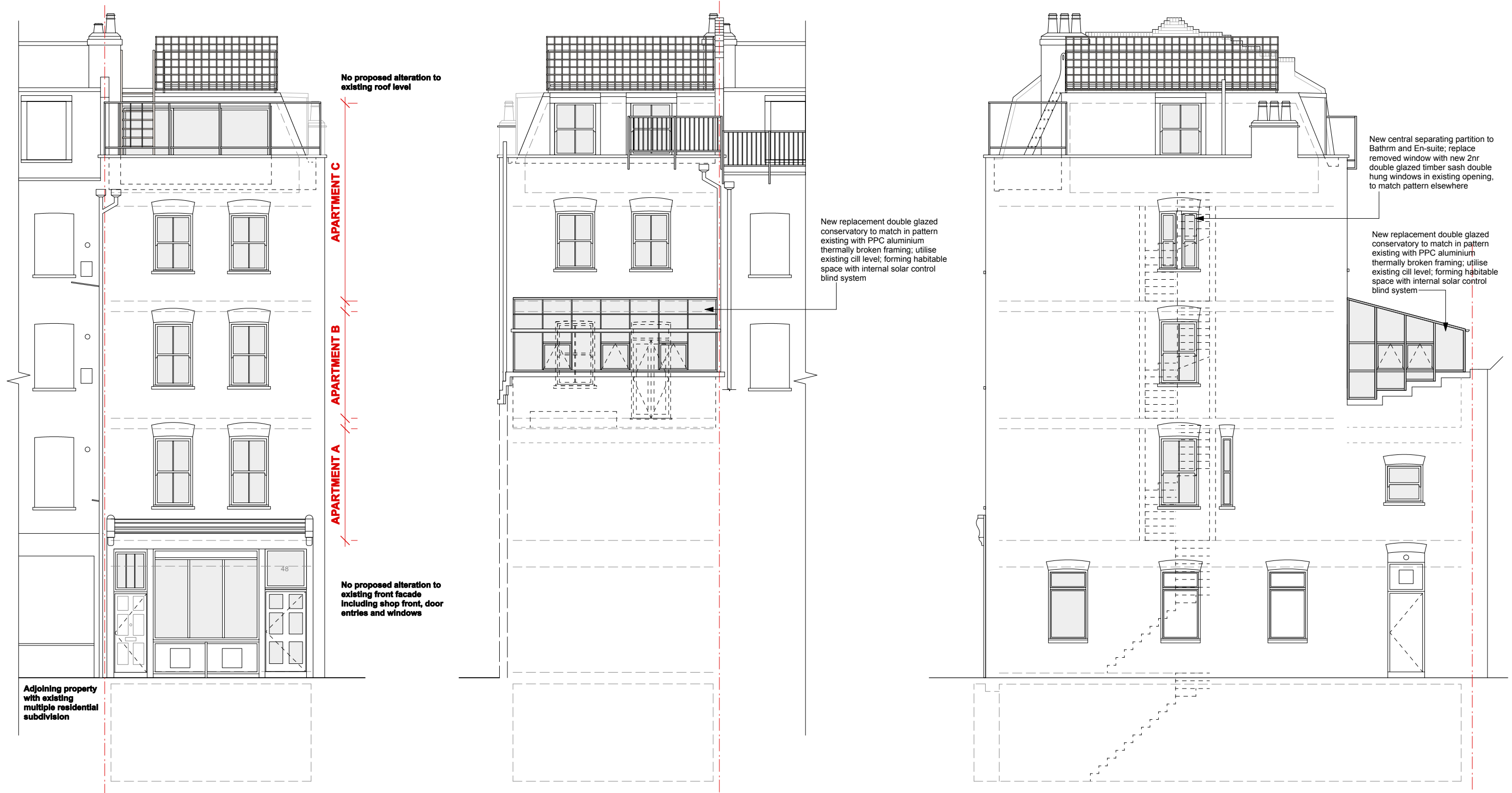
Front Elevation : Proposed Scale 1:100
