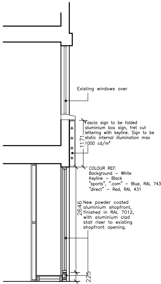
Section B 1:50 Scale
