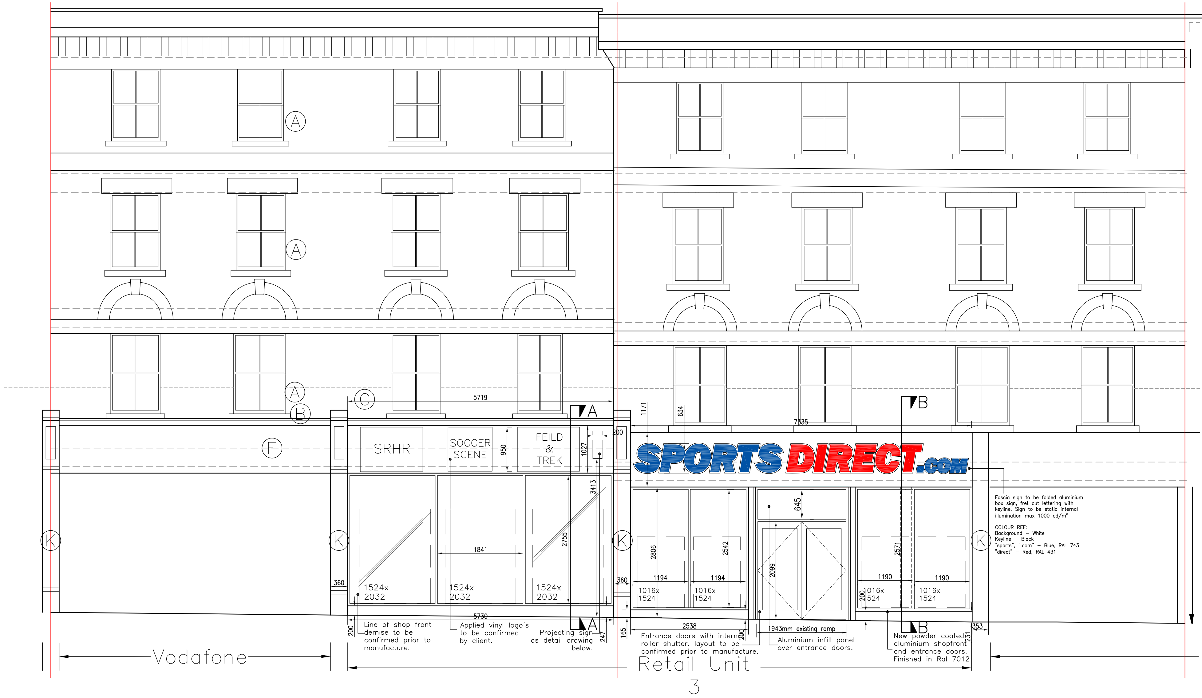
Kilburn High Road Elevation 1:50
