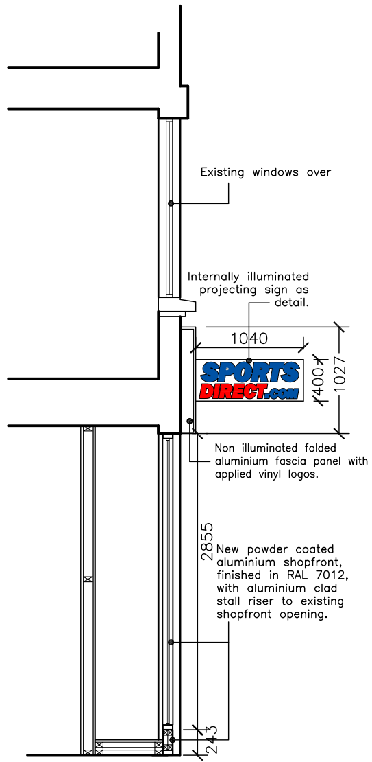
Section A 1:50 scale
