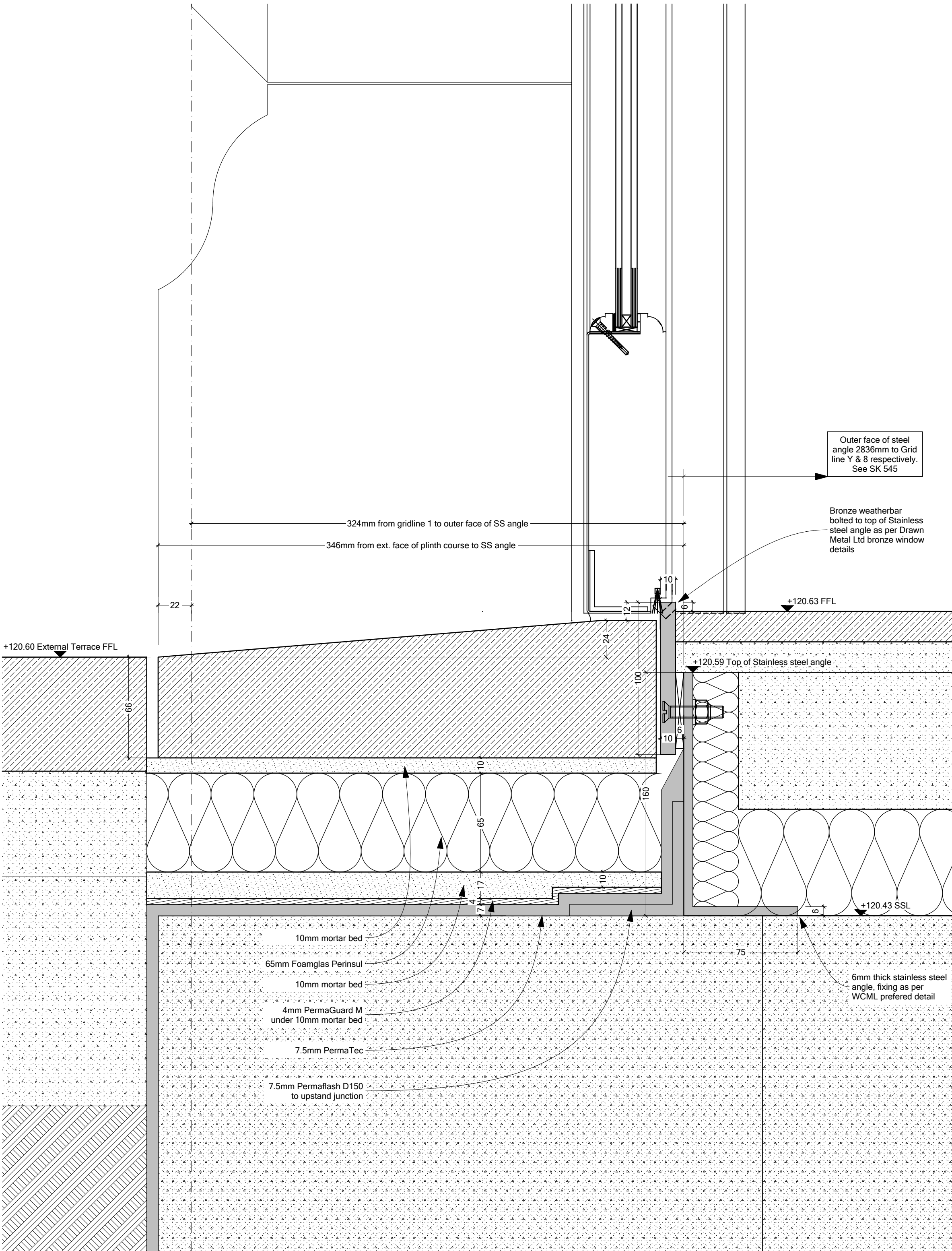
Lower Ground Floor - Stainless Steel Angle Setting Out 1:2
