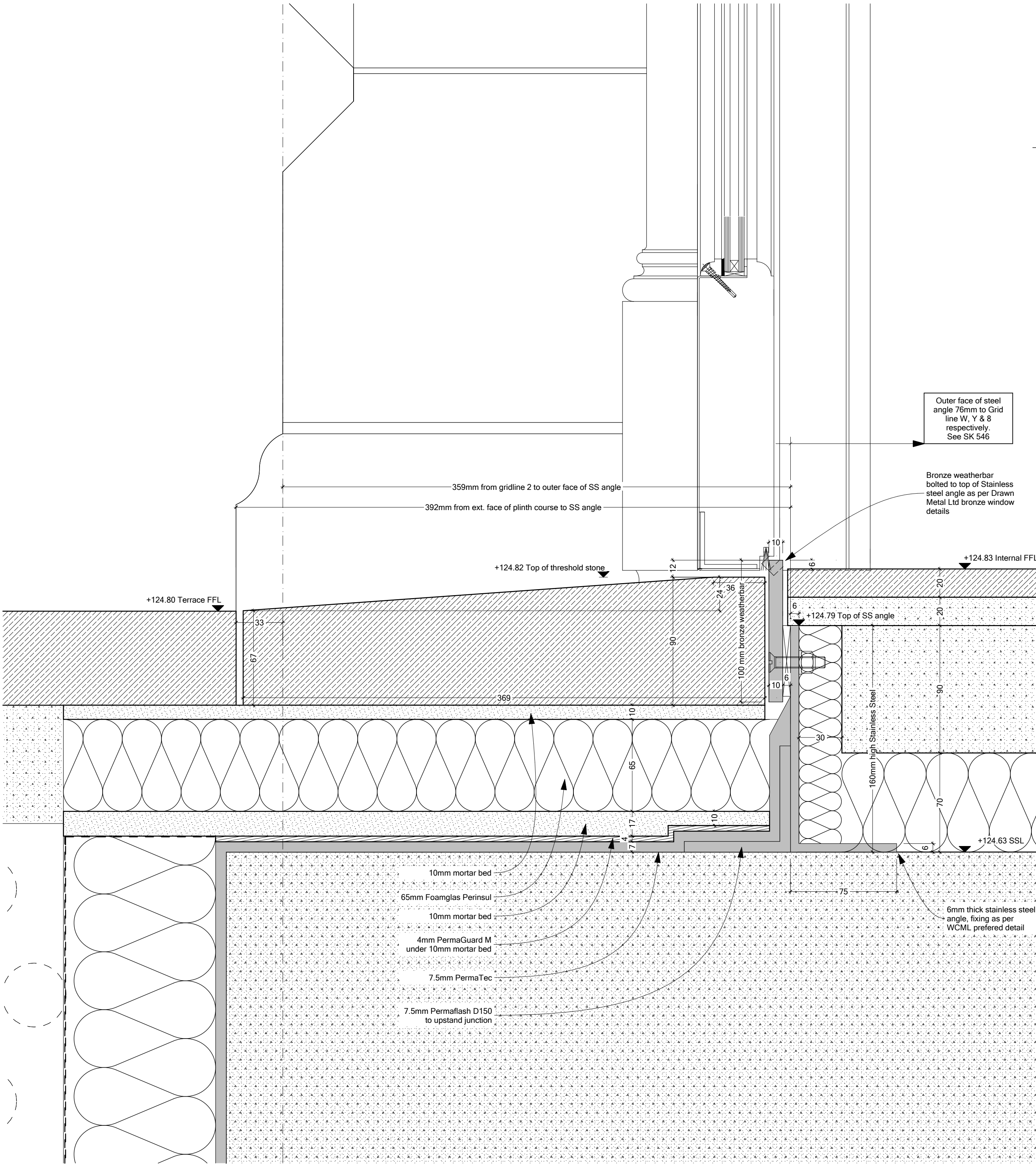
Ground Floor - Stainless Steel Angle Setting Out 1:2
