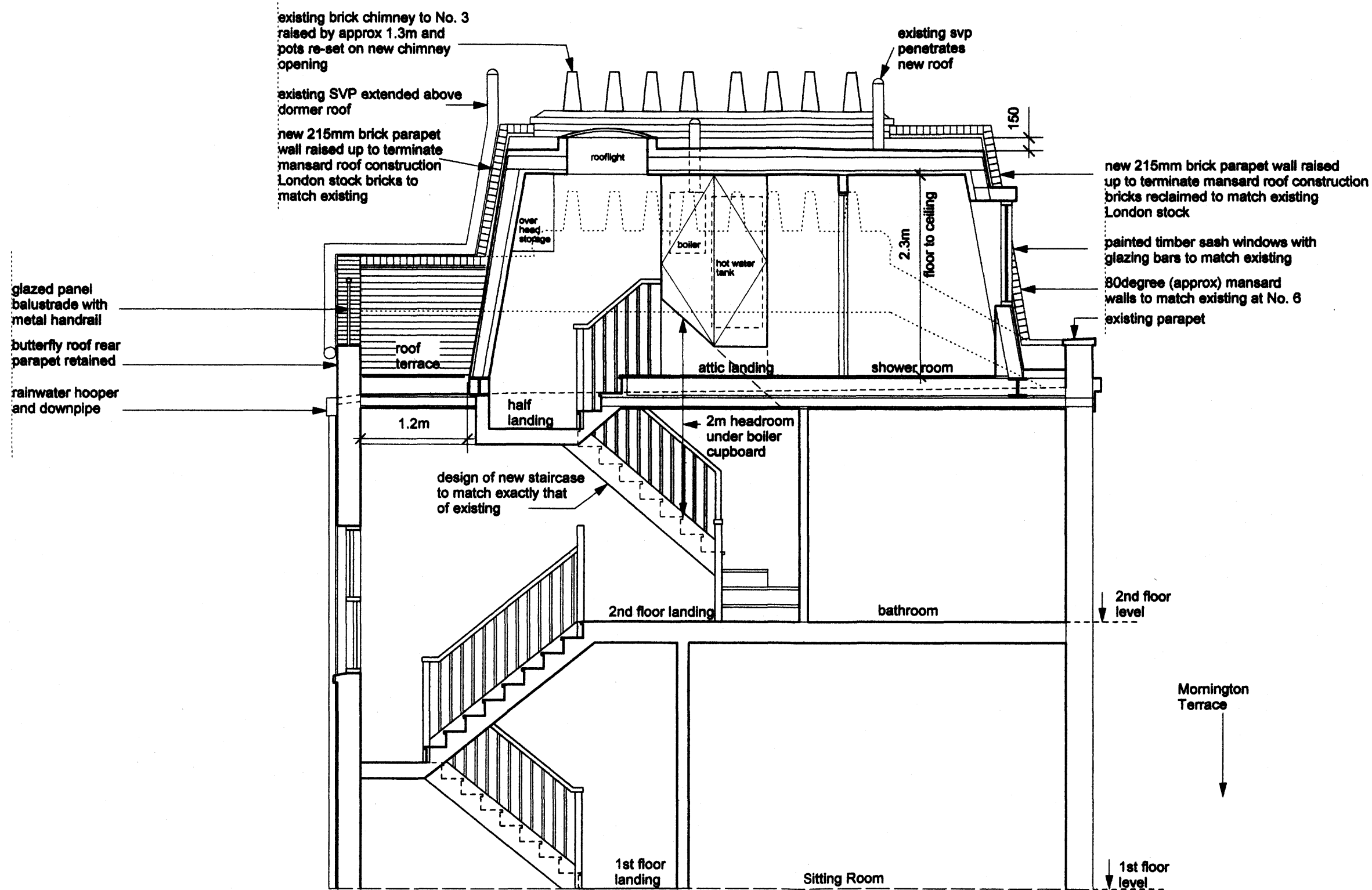
Proposed Section YY
