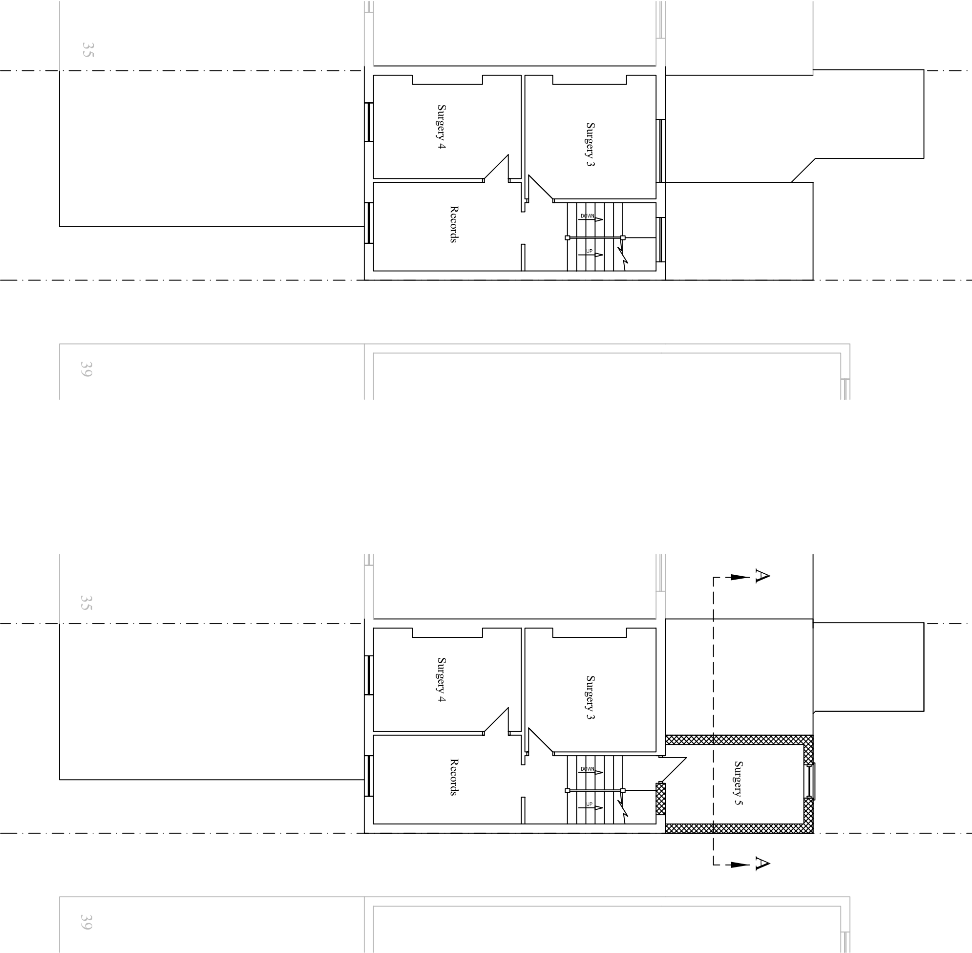
PROPOSED DENTIST FIRST FLOOR LAYOUT
