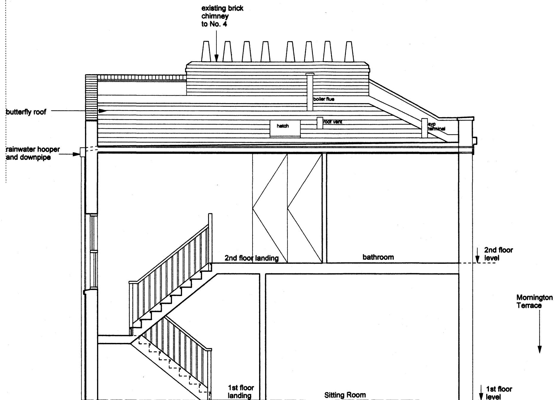
Existing Section YY
