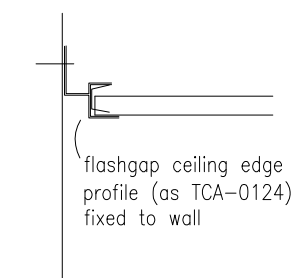
C7 CEILING EDGE typical 600x600 type C1
