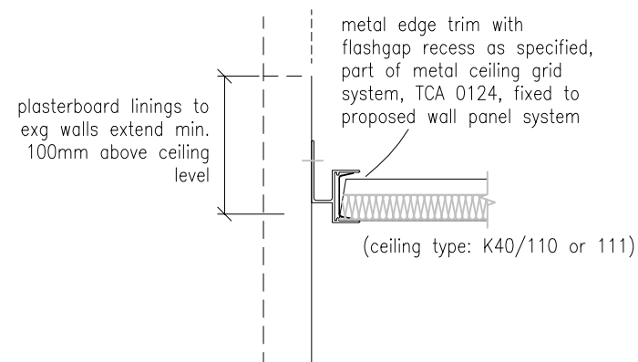
C1 Typical 600x600 suspended metal tile ceiling edge
