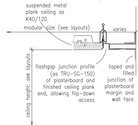
C4 NEW CORRIDOR CEILINGS suspended metal plank junction with plasterboard margin
