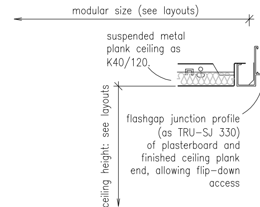
C3 NEW CORRIDOR CEILINGS suspended metal plank junction with partition
