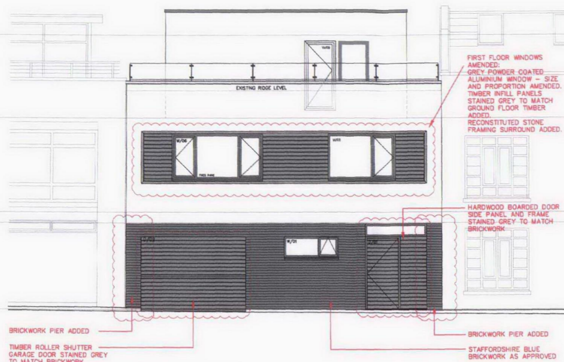
NORTH ELEVATION
