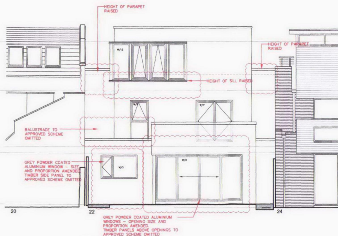
SOUTH ELEVATION
