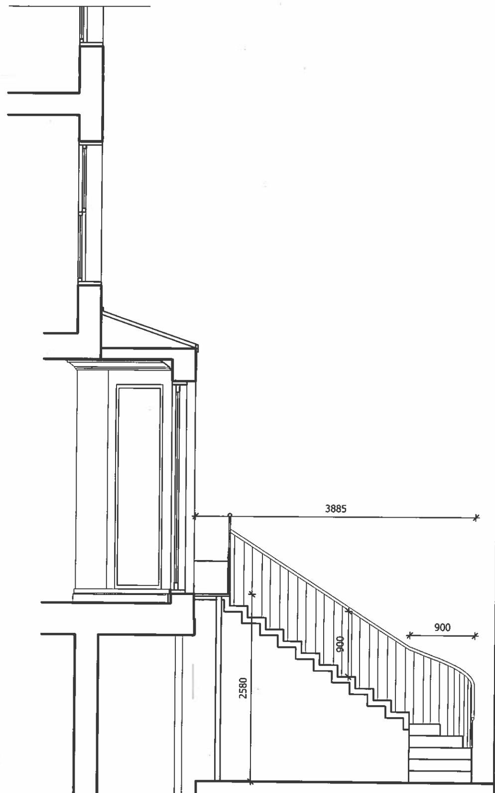
Section A
