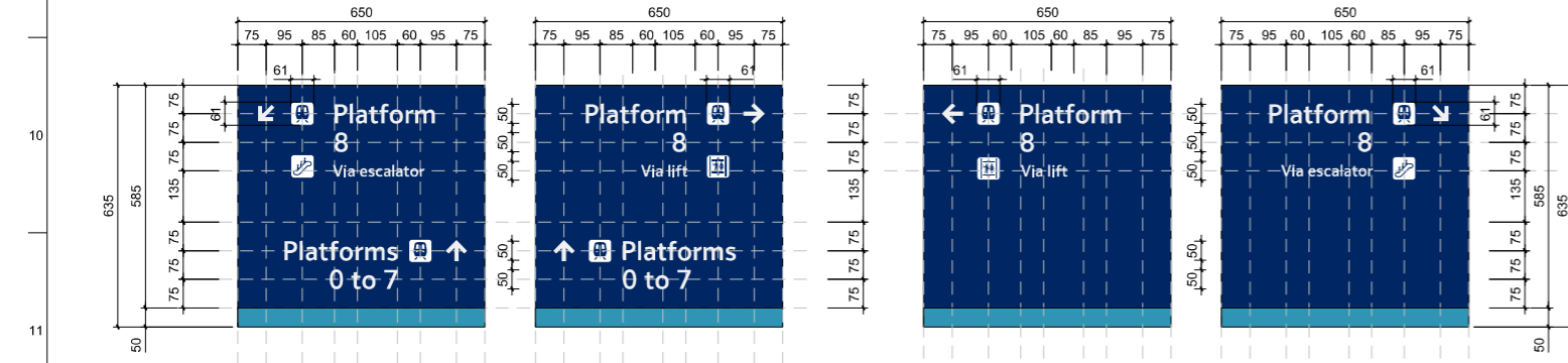
05 TYPOGRAPHIC SETOUT : FOOTBRIDGE COMMS POST WAYFINDING SIGNAGE BOX : PLATFORM 8 - SCALE 1:10
