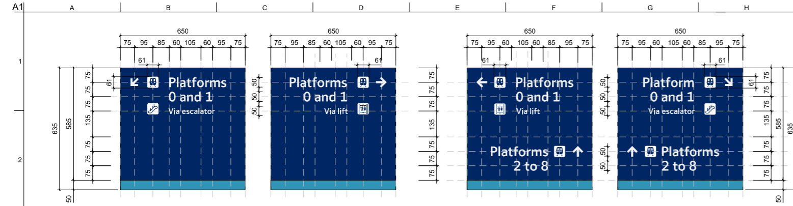
01 TYPOGRAPHIC SETOUT : FOOTBRIDGE COMMS POST WAYFINDING SIGNAGE BOX : PLATFORM 0/1 - SCALE 1:10
