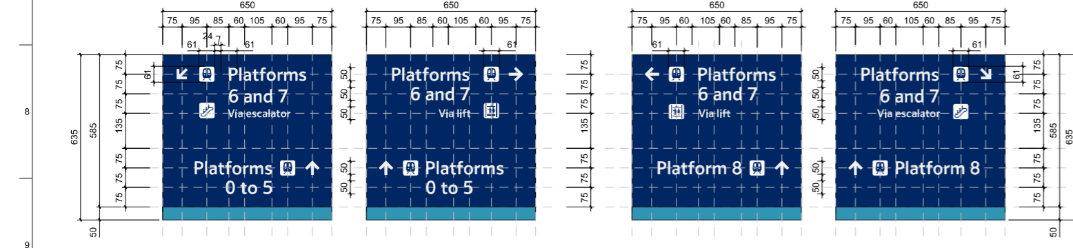
04 TYPOGRAPHIC SETOUT : FOOTBRIDGE COMMS POST WAYFINDING SIGNAGE BOX : PLATFORM 6/7 - SCALE 1:10
