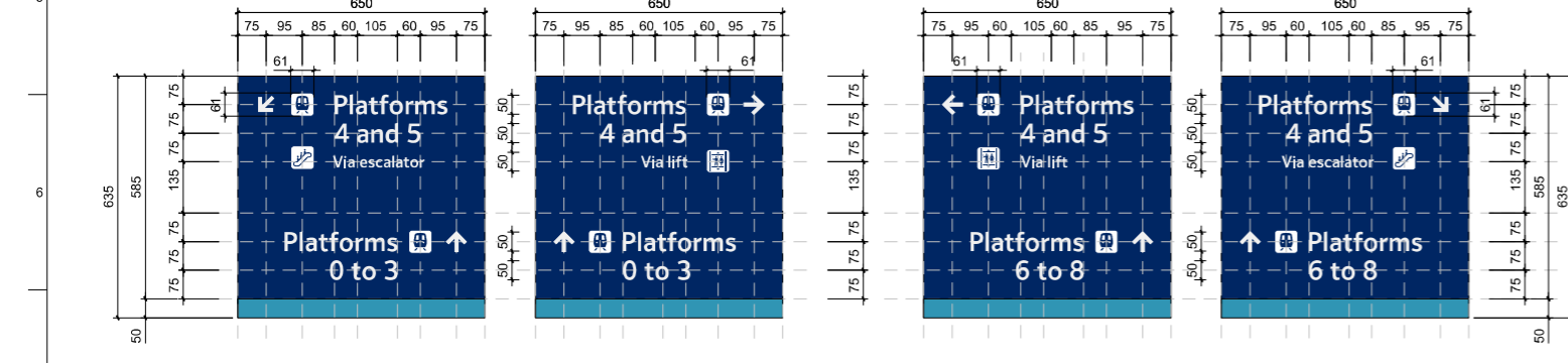
03 TYPOGRAPHIC SETOUT : FOOTBRIDGE COMMS POST WAYFINDING SIGNAGE BOX : PLATFORM 4/5 - SCALE 1:10
