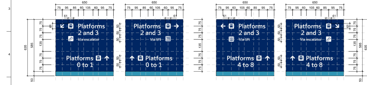
02 TYPOGRAPHIC SETOUT : FOOTBRIDGE COMMS POST WAYFINDING SIGNAGE BOX : PLATFORM 2/3 - SCALE 1:10
