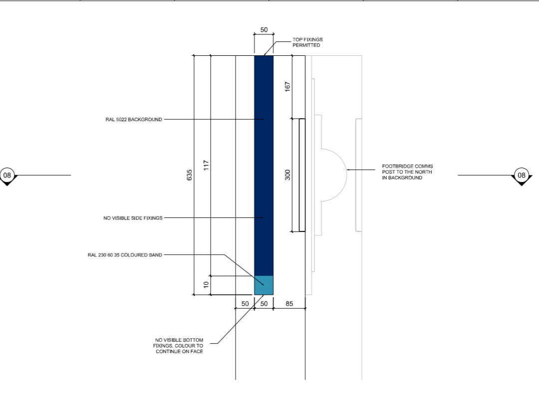
06 DETAILED SECTION THRU WAYFINDING BOX - SCALE 1:5
