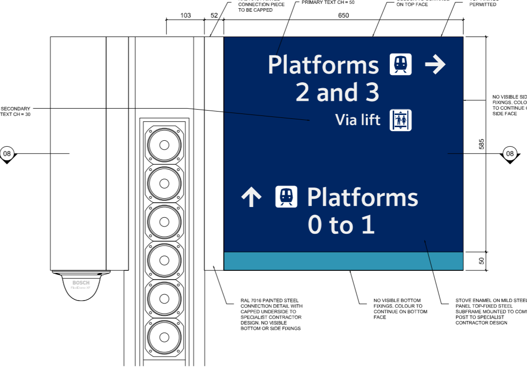
07 TYPICAL FRONT ELEVATION - SCALE 1:5
