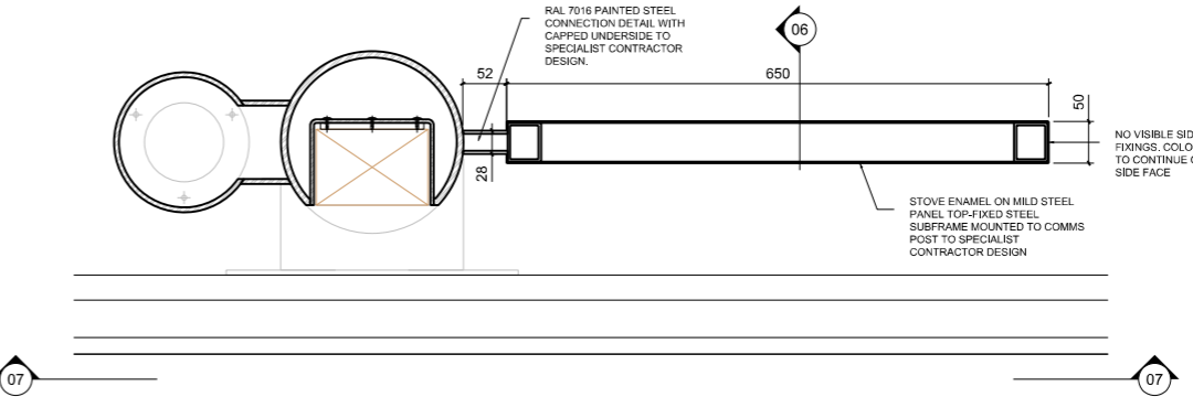
08 DETAILED PLAN - SCALE 1:5
