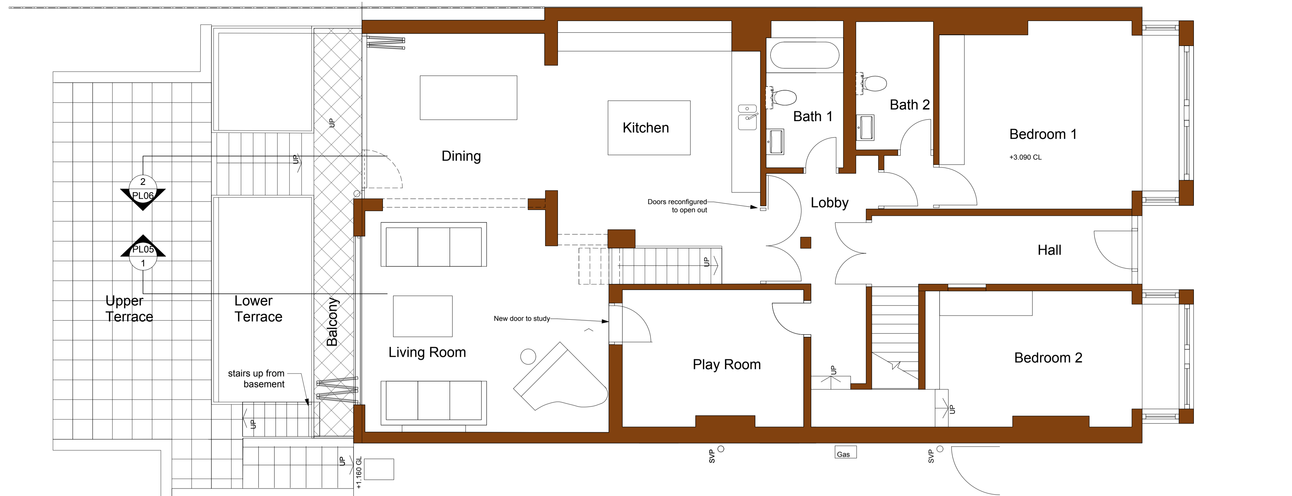
1 Proposed Upper Ground Floor
