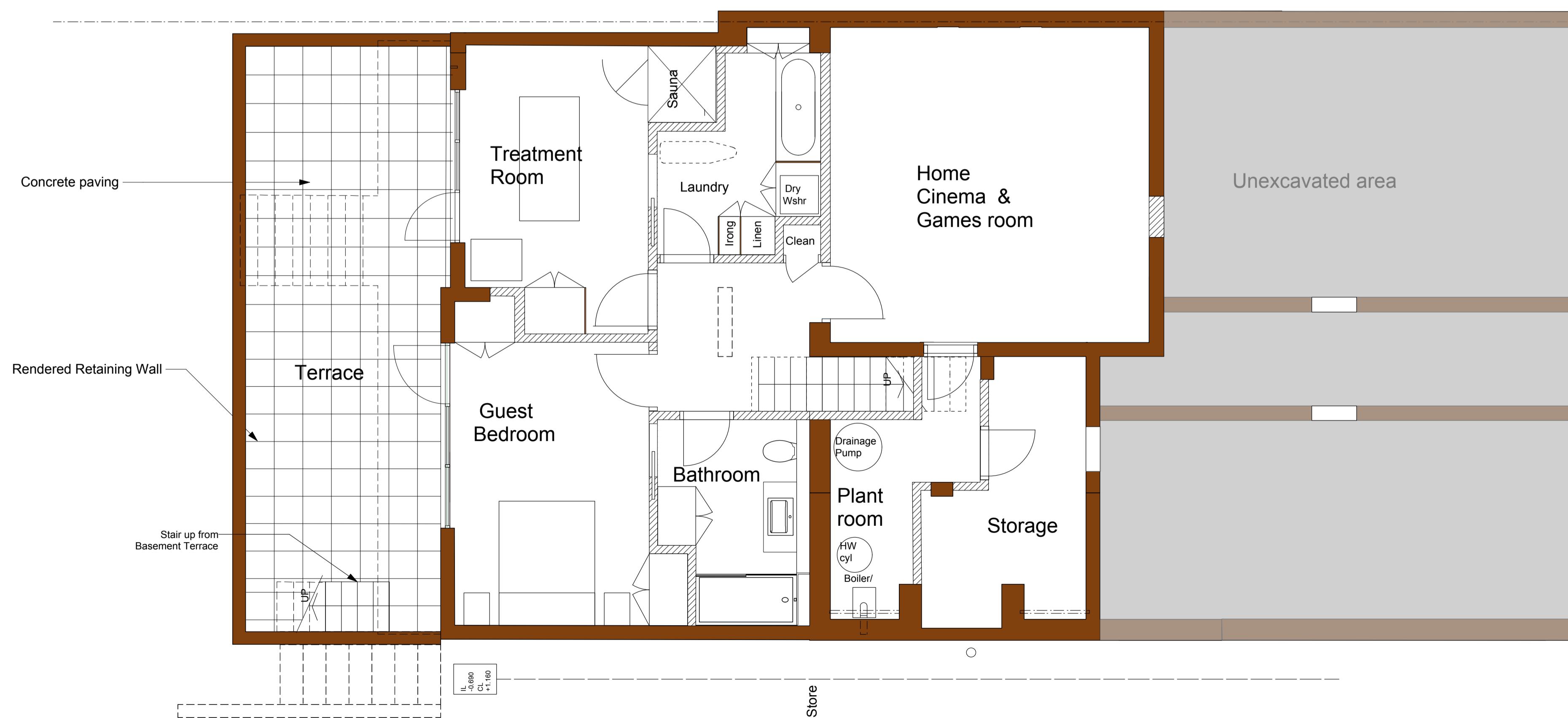
2 Proposed Lower Ground Floor
