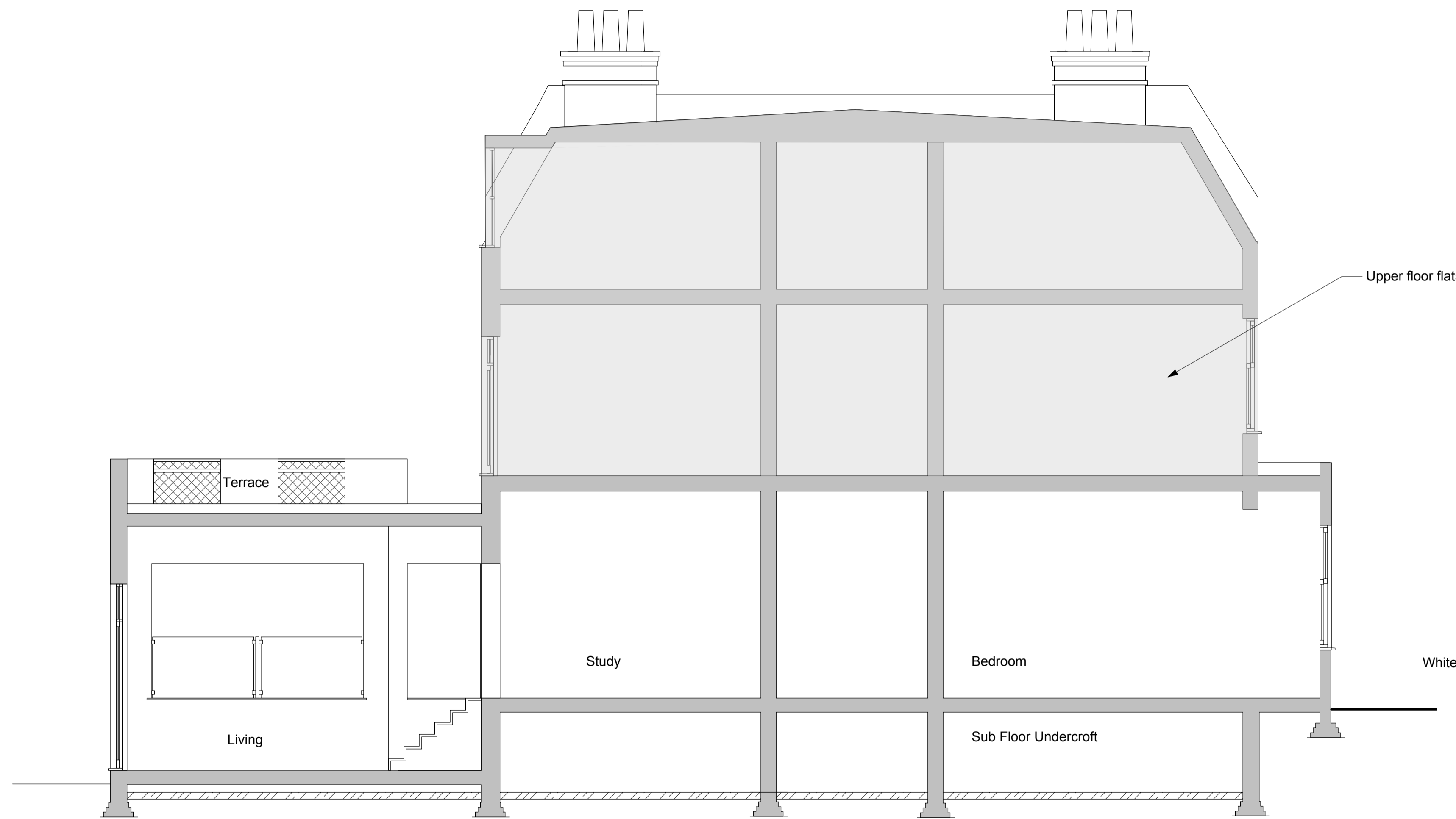
1 Existing Section
