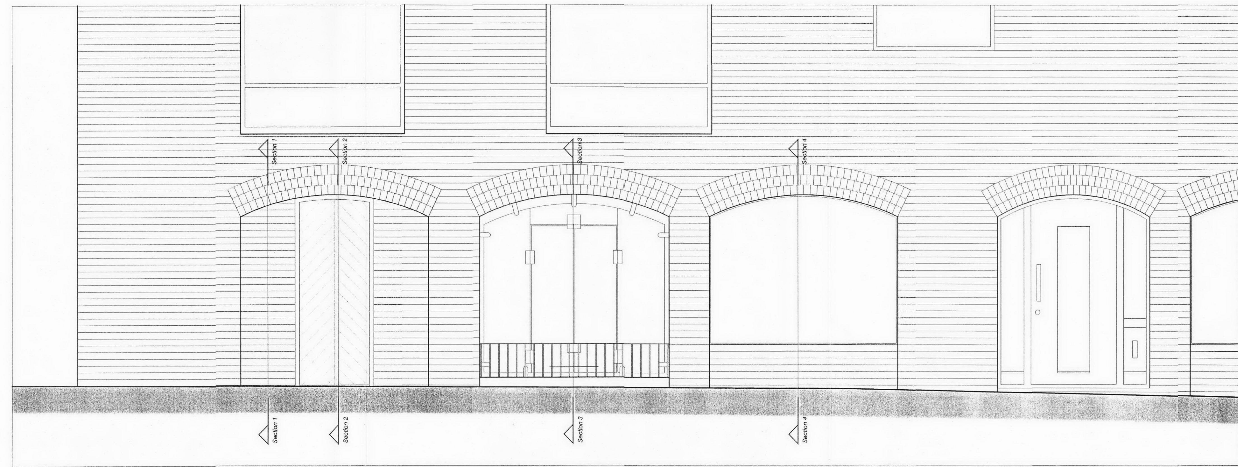
ELEVATION SCALE 1:25 @ A1
