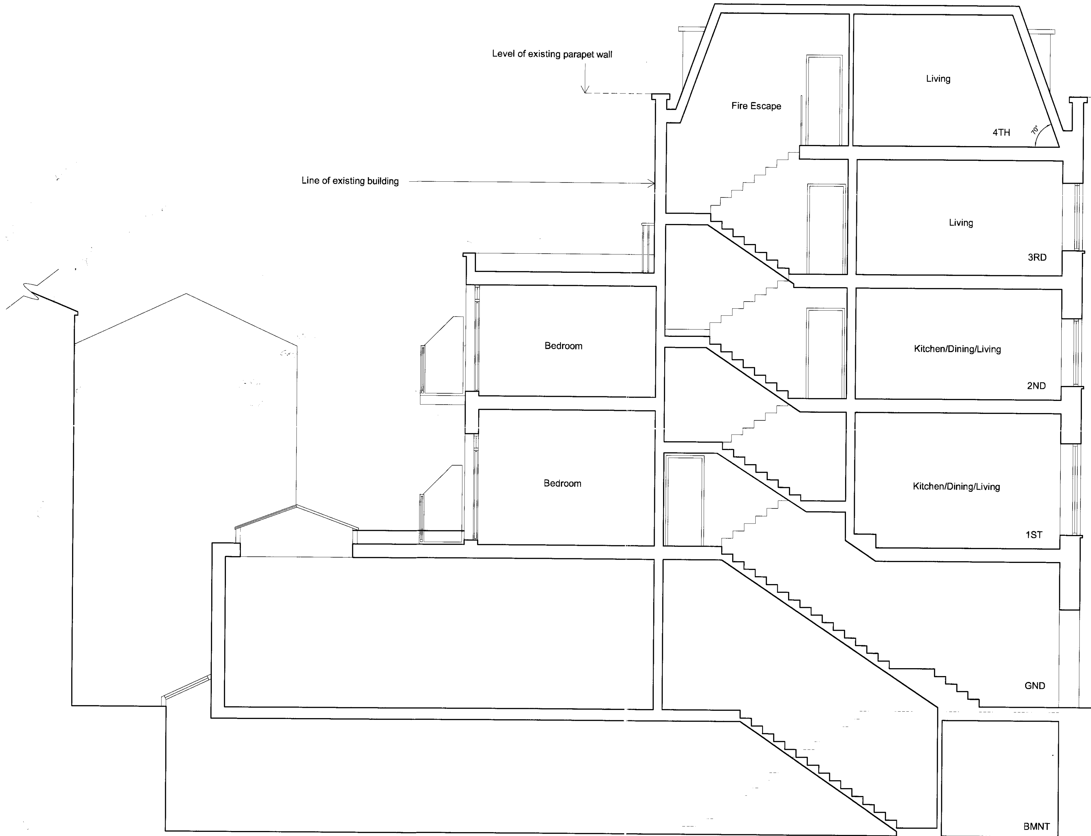
Section AA
