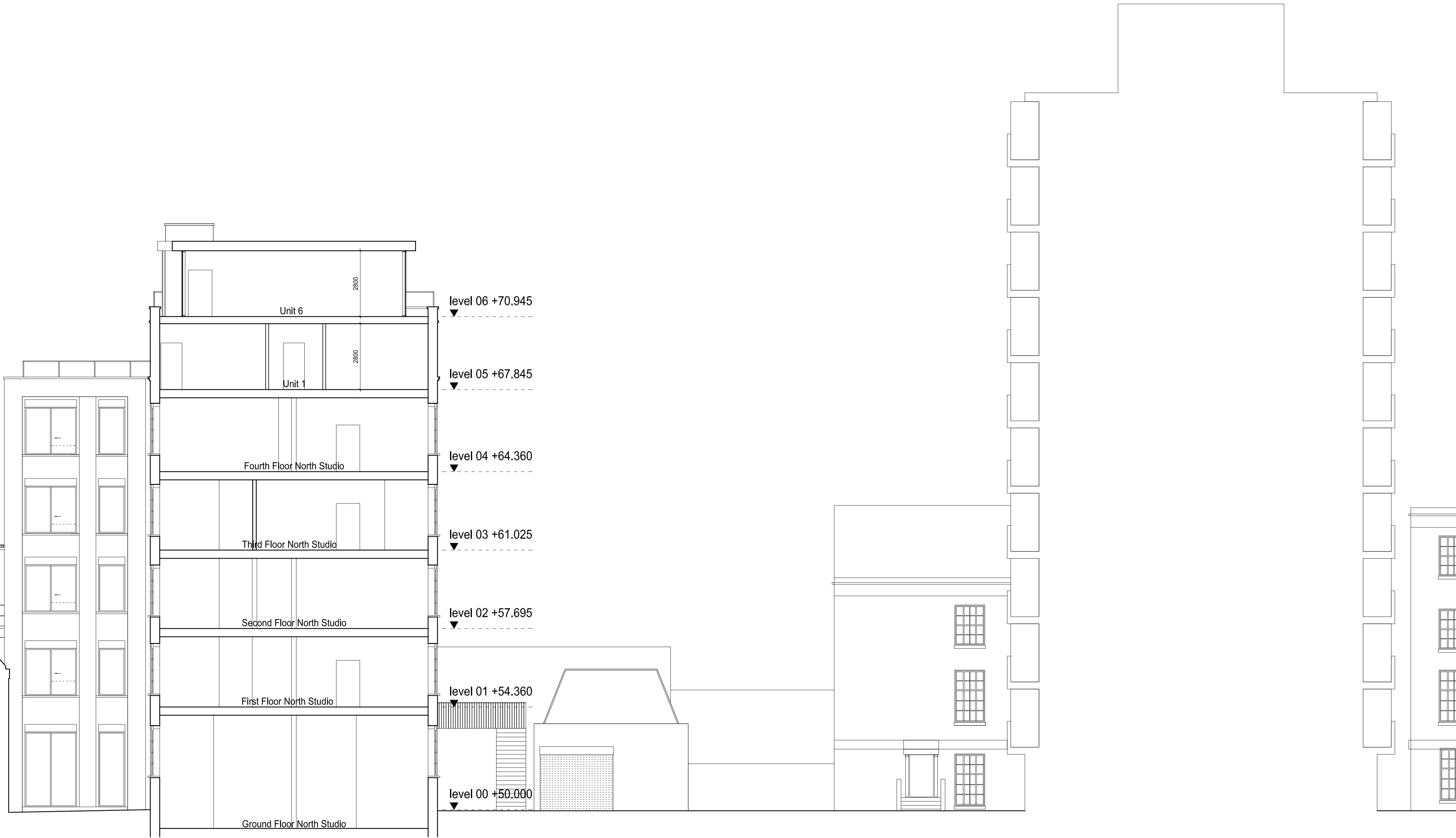
PROPOSED C-C' SECTION
