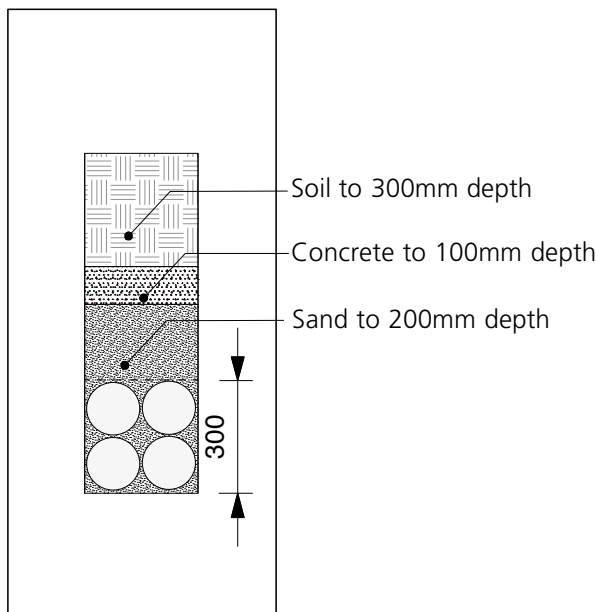
Trench Detail Scale 1:20
