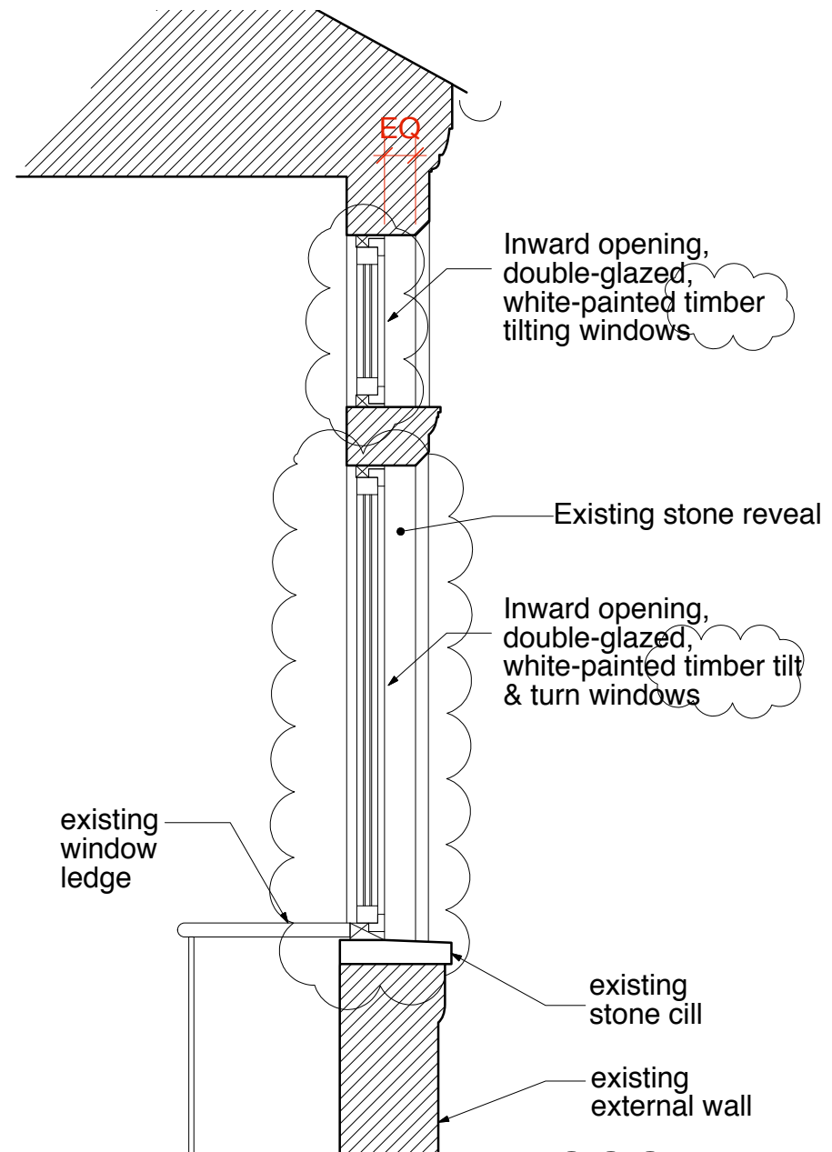
Section Detail of a Proposed Timber Windows 1:20
