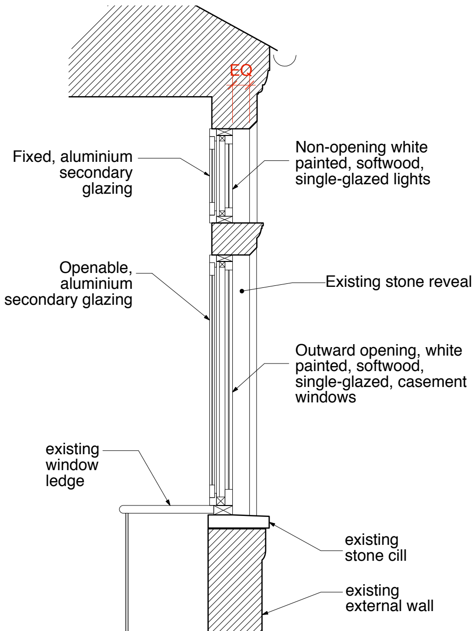
Typical Section Detail of Existing Casement Window 1:20
