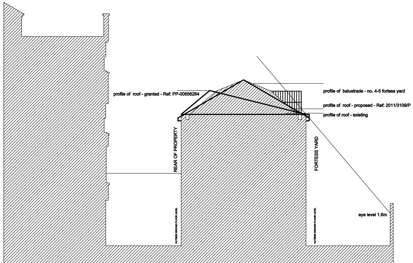
SECTION through context
