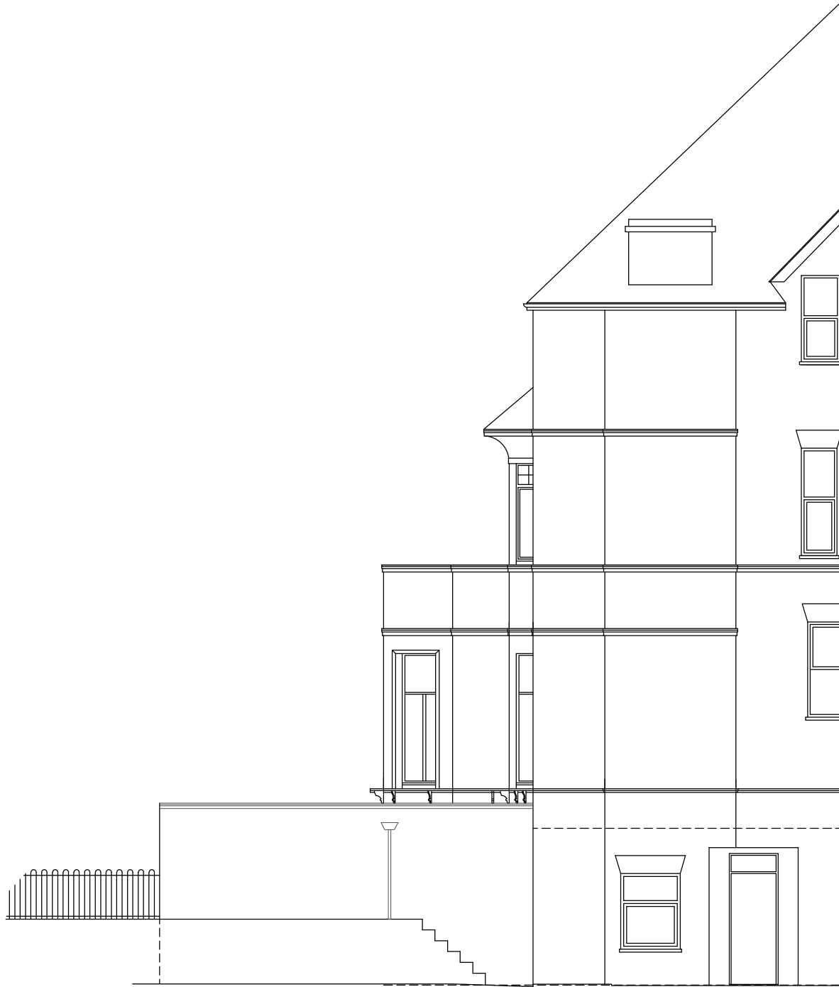
PROPOSED GABLE ELEVATION
