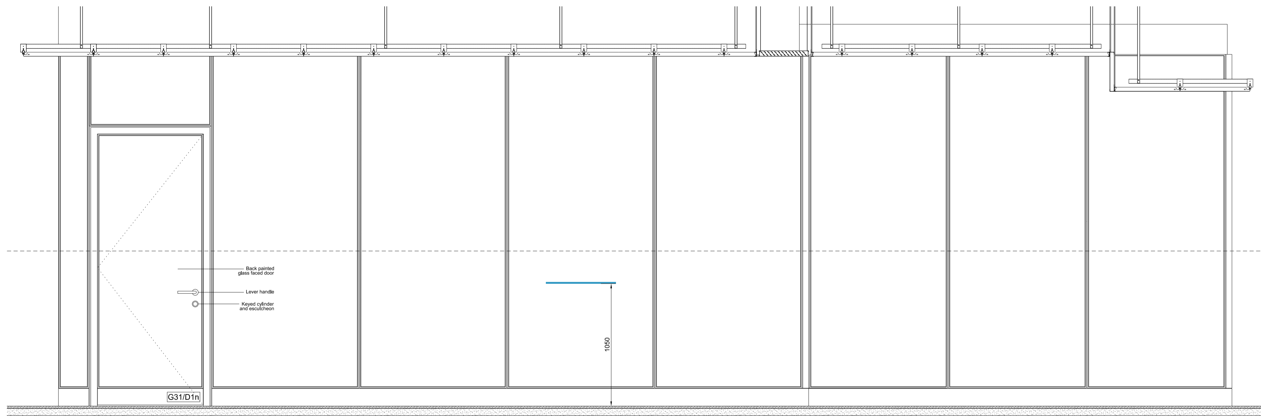
03 PUBLIC TOILET CORRIDOR ELEVATION SCALE 1:20
