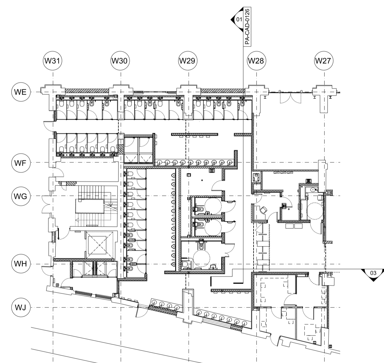
00 PUBLIC TOILET KEY PLAN SCALE 1:200
